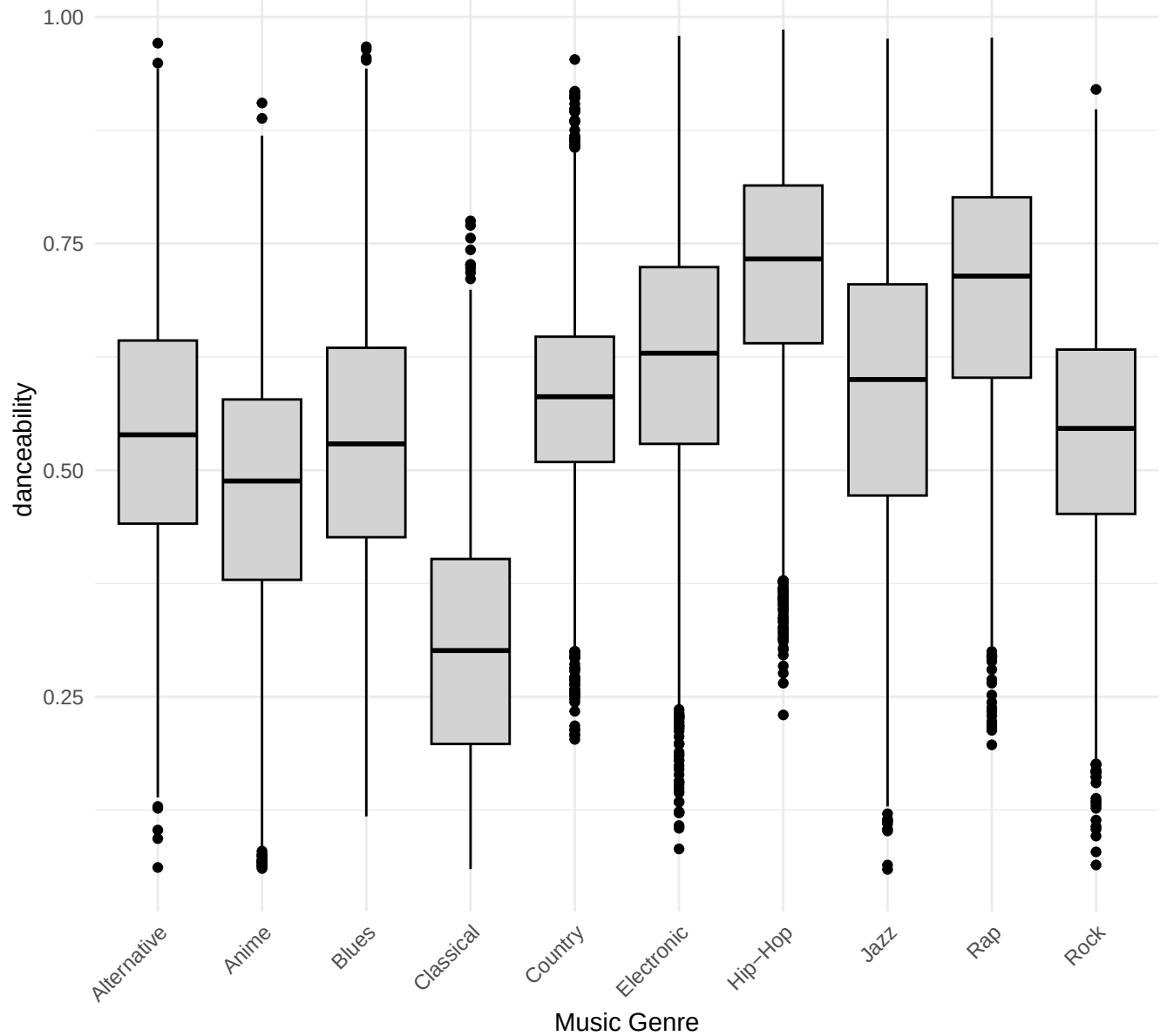
Boxplot of danceability by Genre
