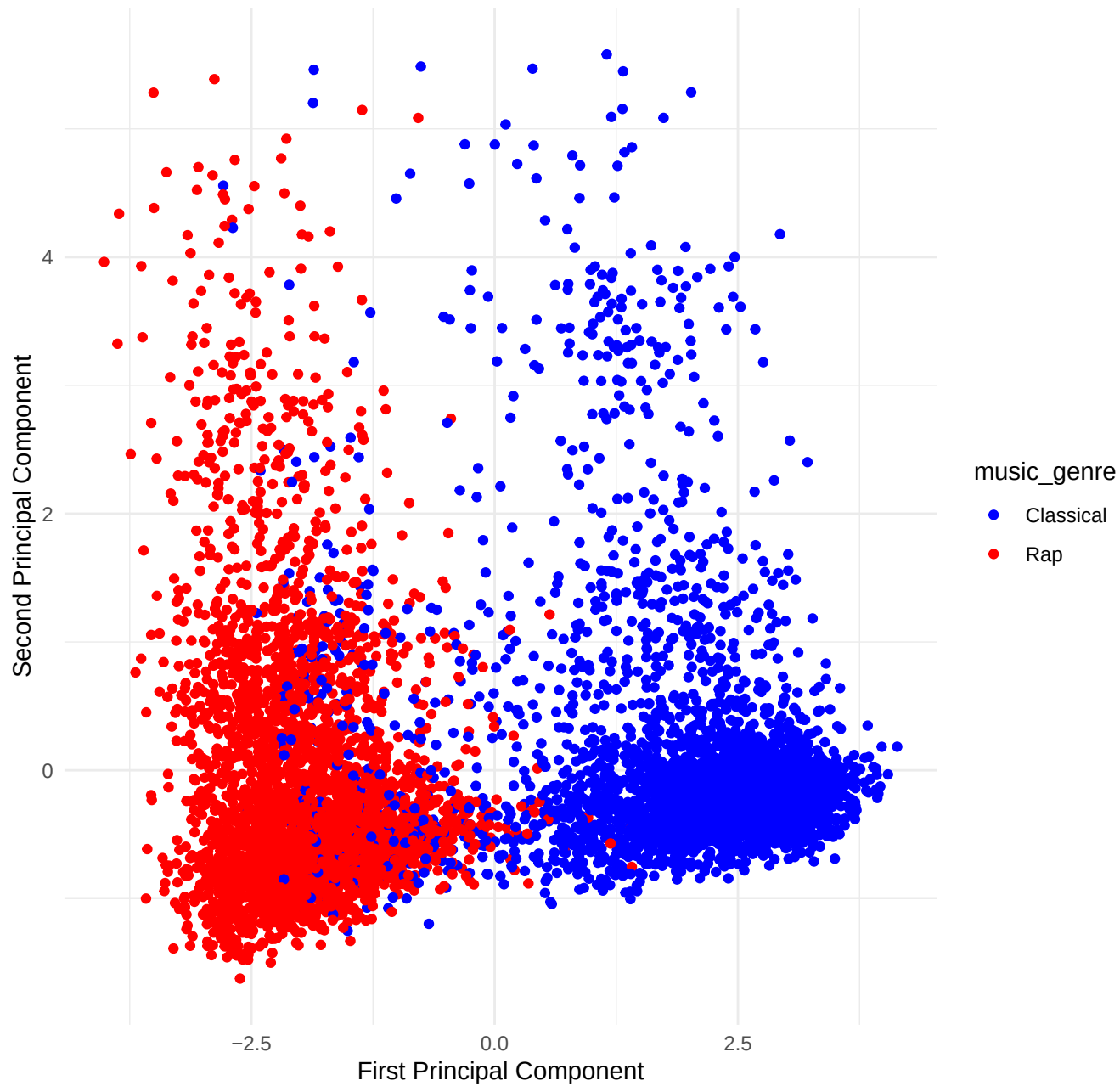
PCA: First vs. Second Principal Component
