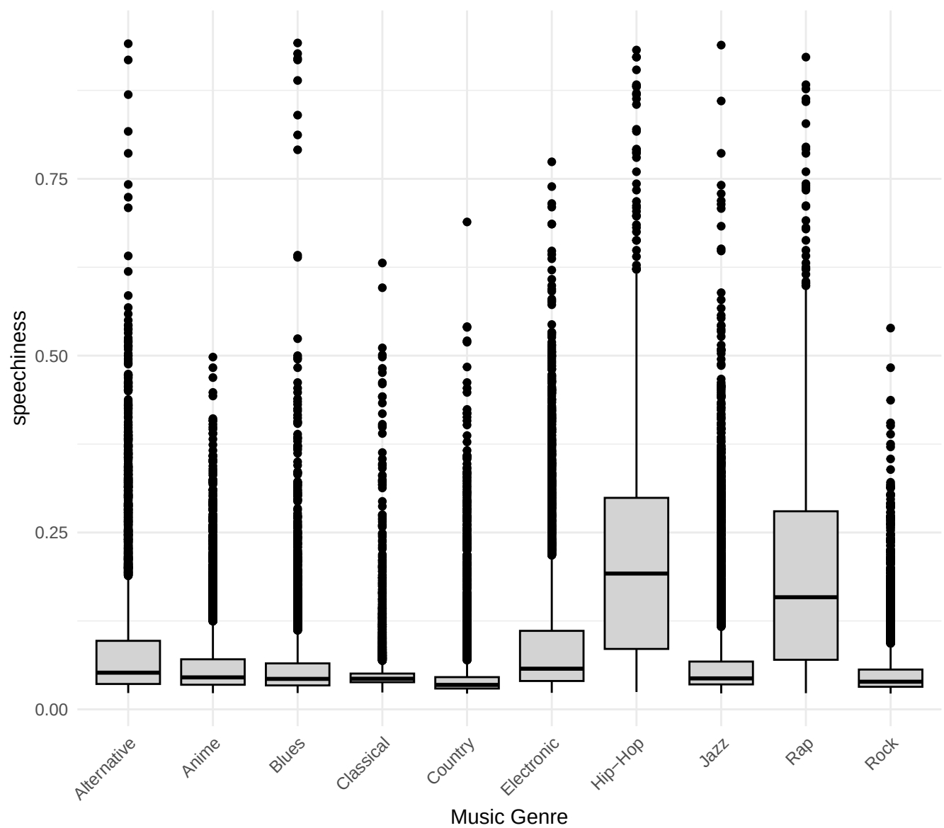
Boxplot of speechiness by Genre
