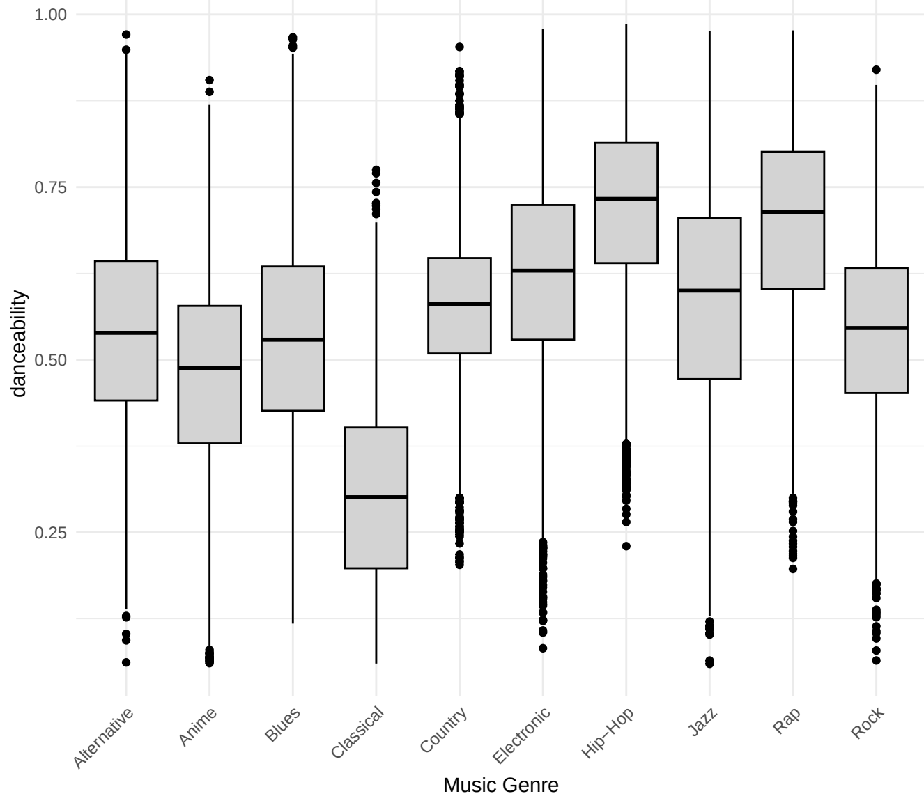
Boxplot of danceability by Genre
