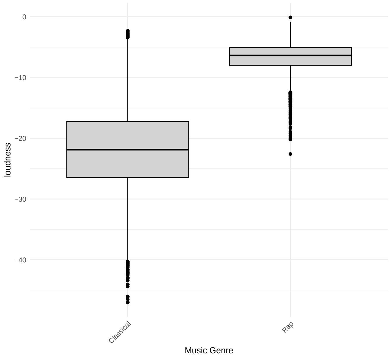
Boxplot of loudness by Genre
