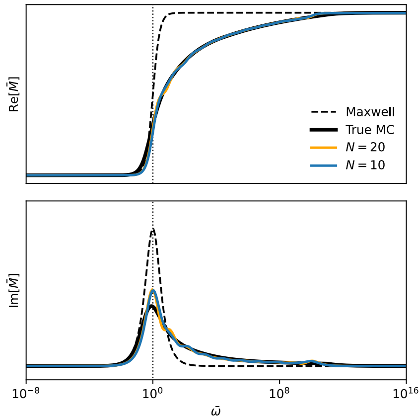
(B) Fitting Results
