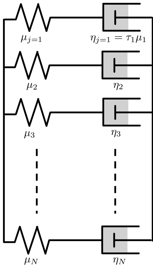
(A) Generalized Maxwell
