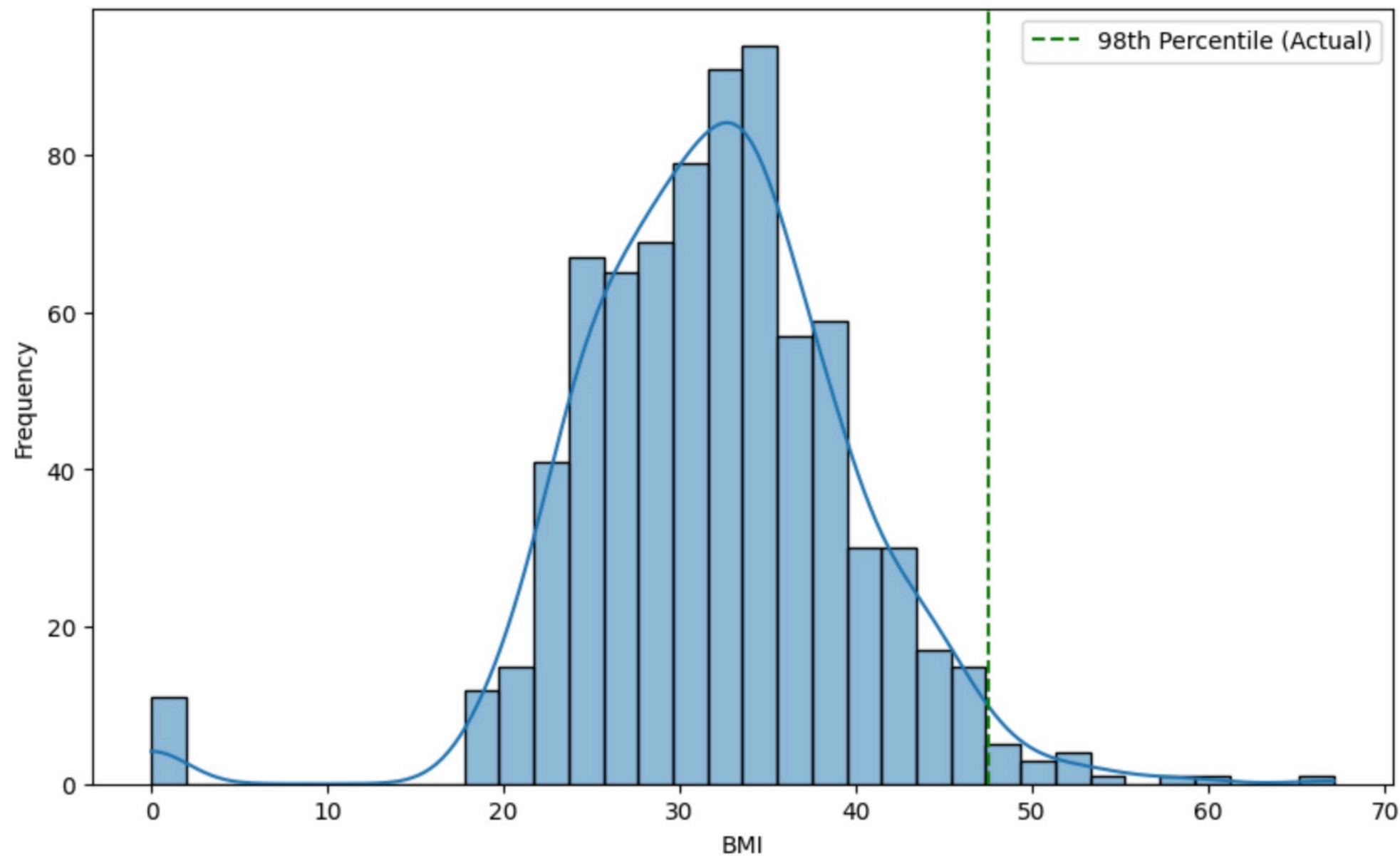
Distribution of BMI in Full Data with 98th Percentile (Actual)
