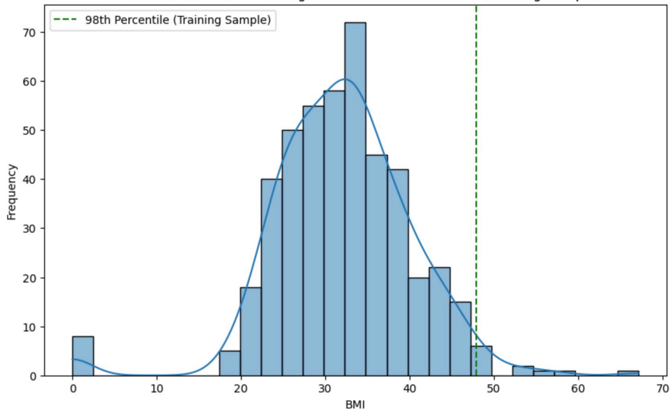
Distribution of BMI in Training Data with 98th Percentile (Training Sample)
