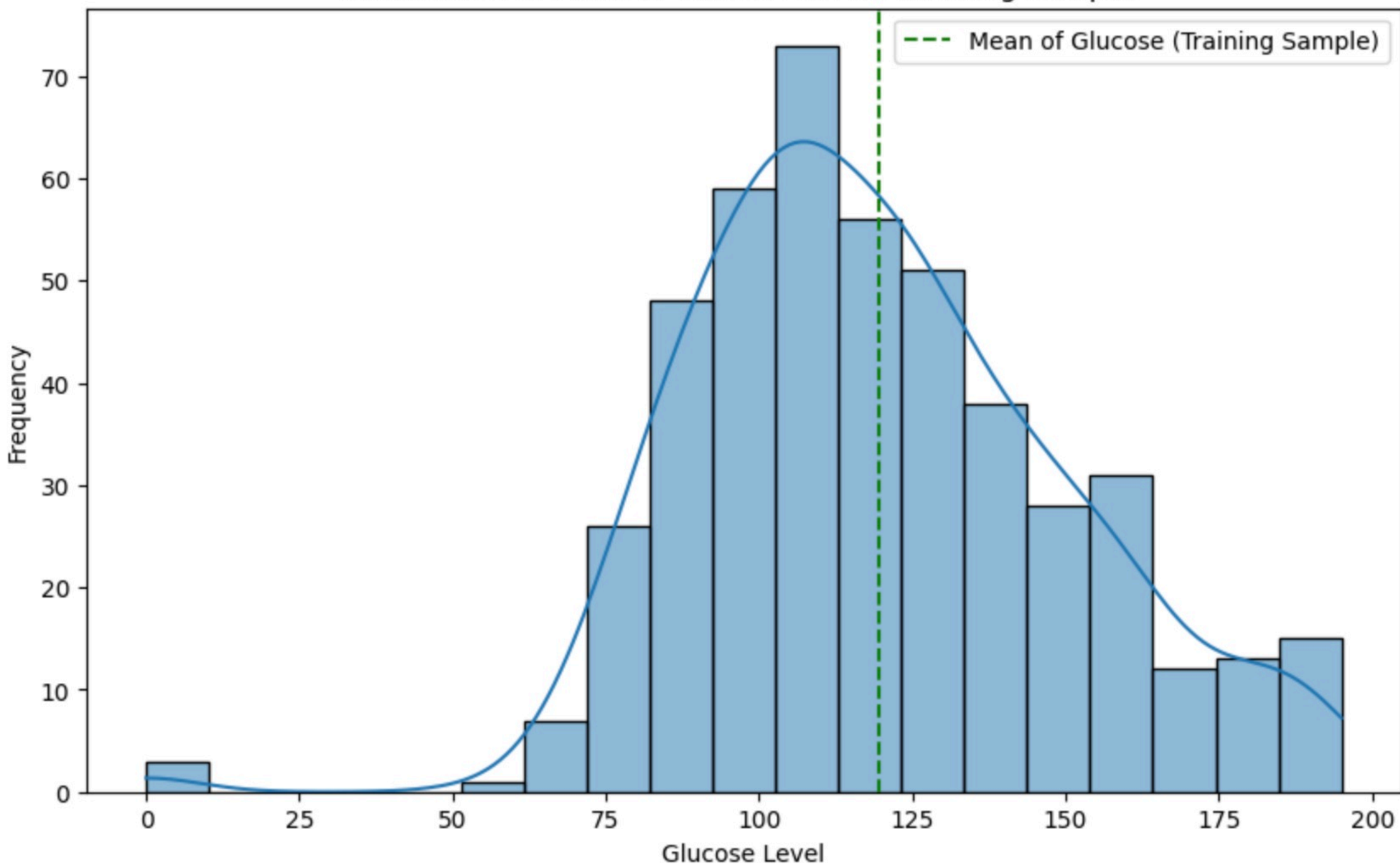
Distribution of Mean of Glucose Levels (Training Sample)
