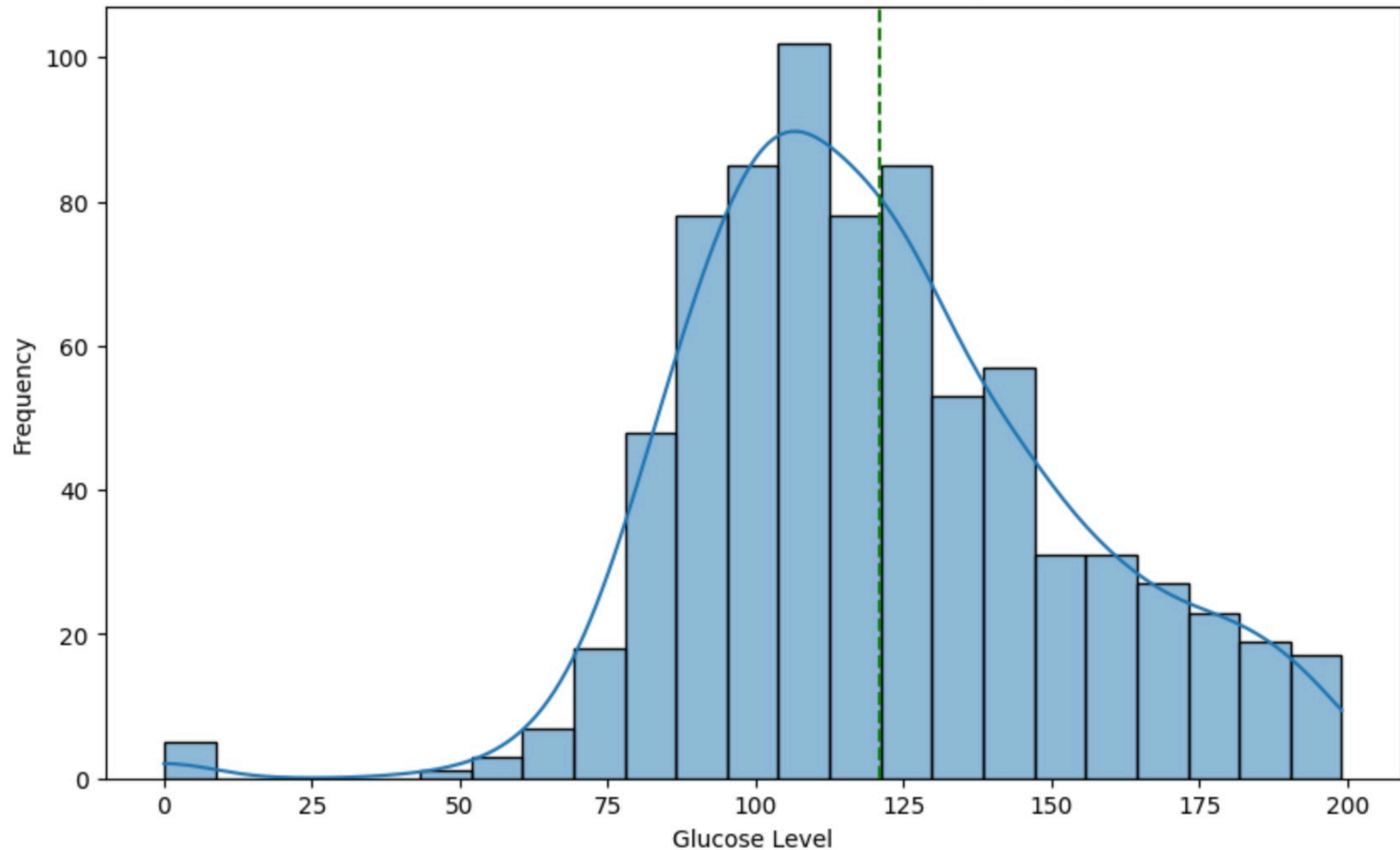
Distribution of Mean of Glucose Levels (Actual)
