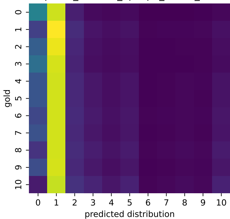
prefix_unnorm_eps1p0_seed0_fs5
