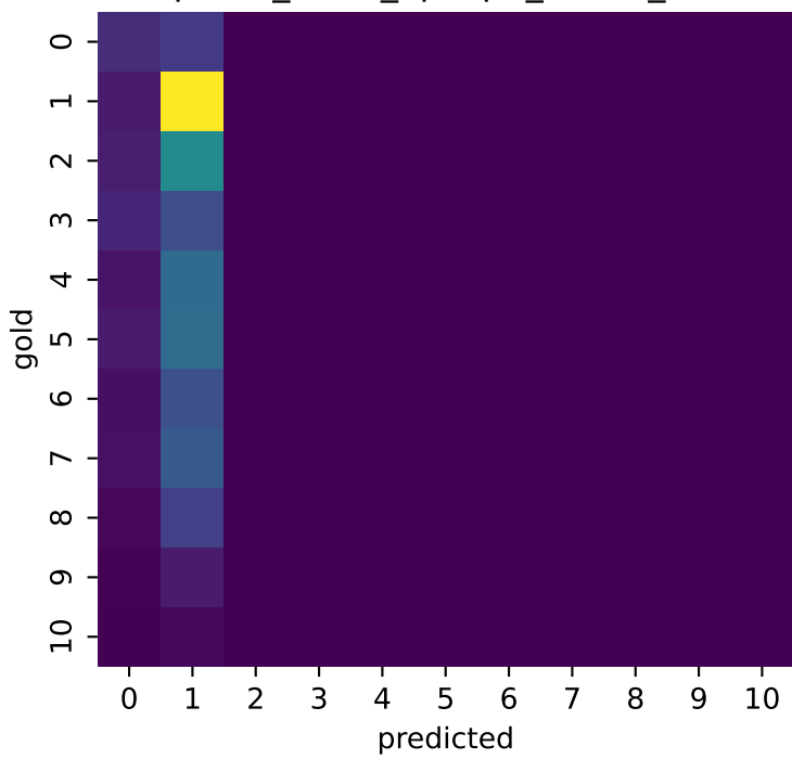
prefix_unnorm_eps1p0_seed0_fs5
