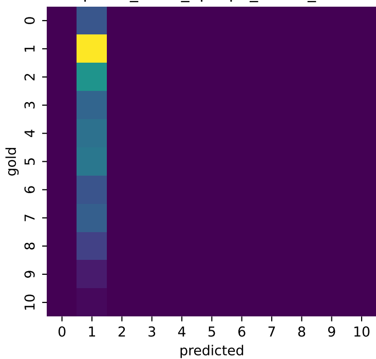
prefix_unnorm_eps0p1_seed0_fs5
