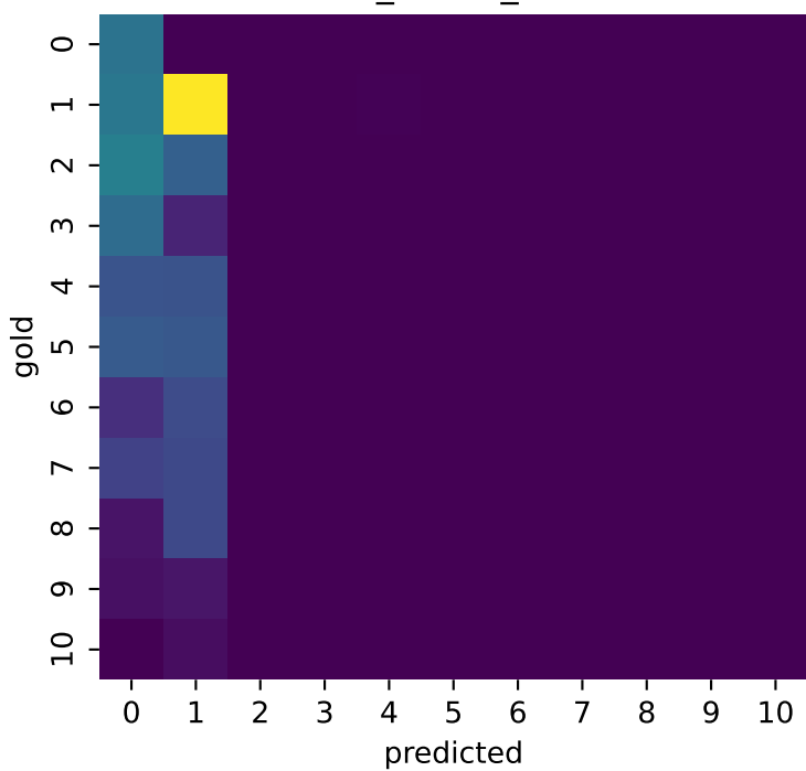
prefix_norm_eps1p0_seed0_fs5
