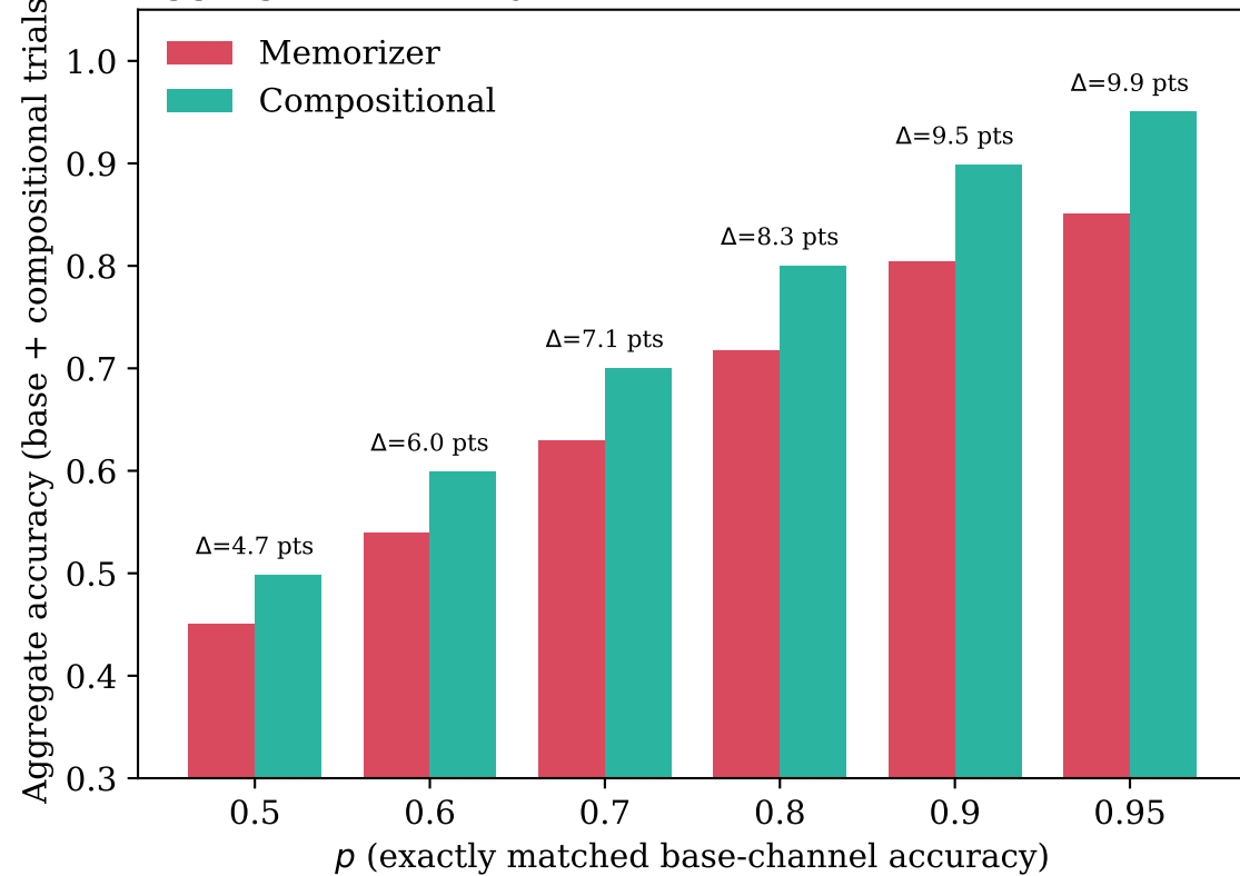
Aggregate accuracy compresses the held-out difference
