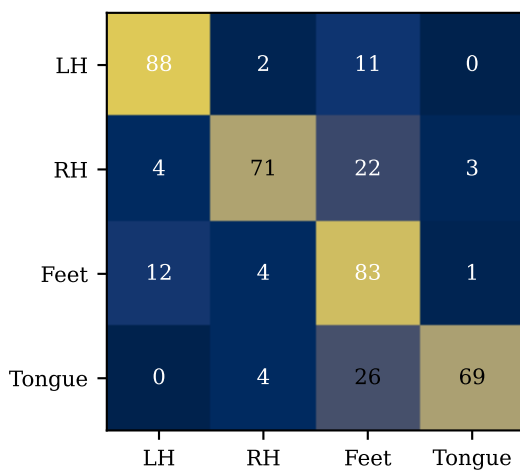
S8: acc 0.77, \kappa 0.70
