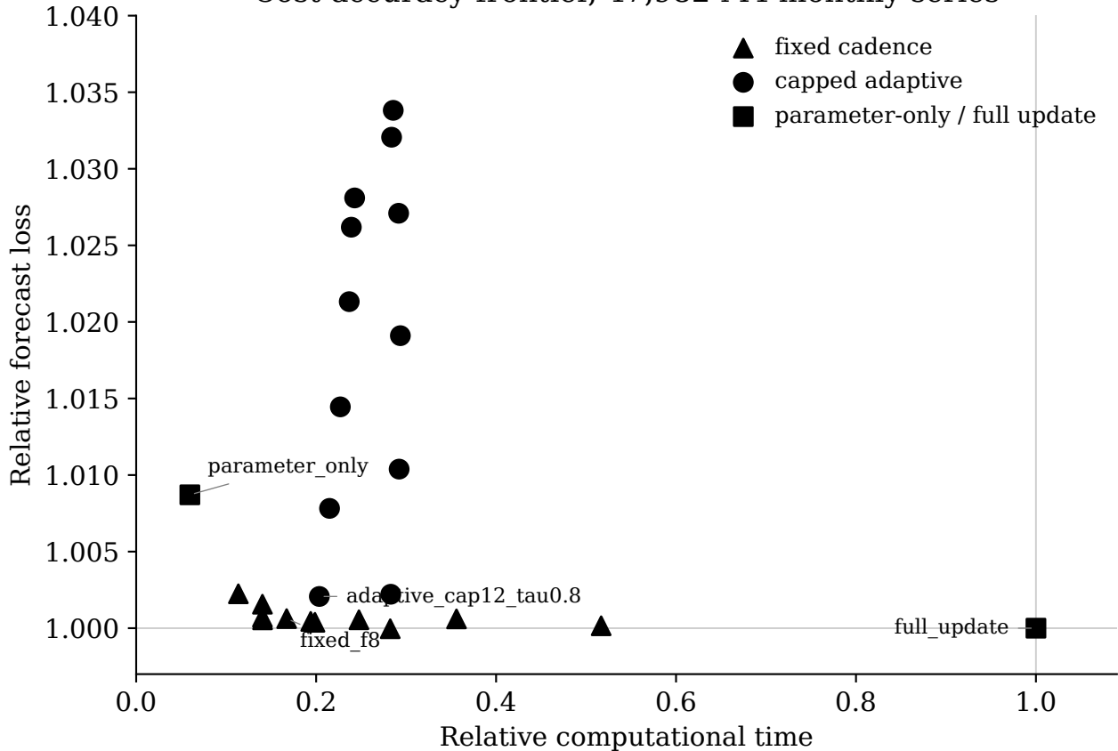
Cost-accuracy frontier, 47,982 M4 monthly series
