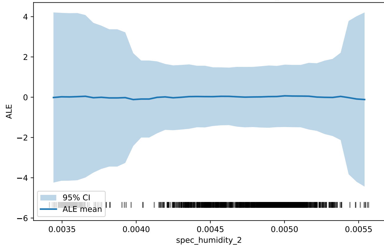
ALE for feature spec_humidity_2
