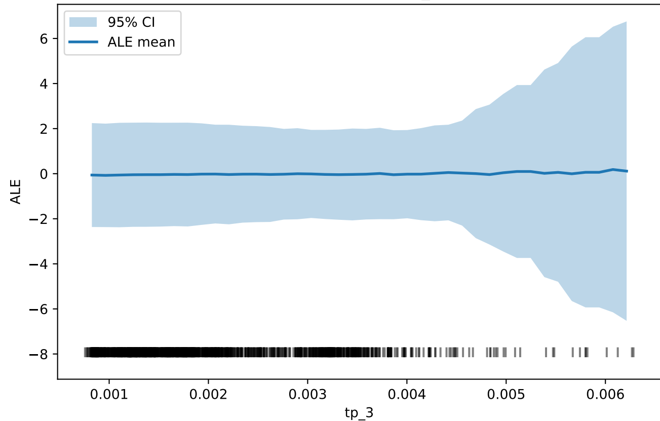
ALE for feature tp_3
