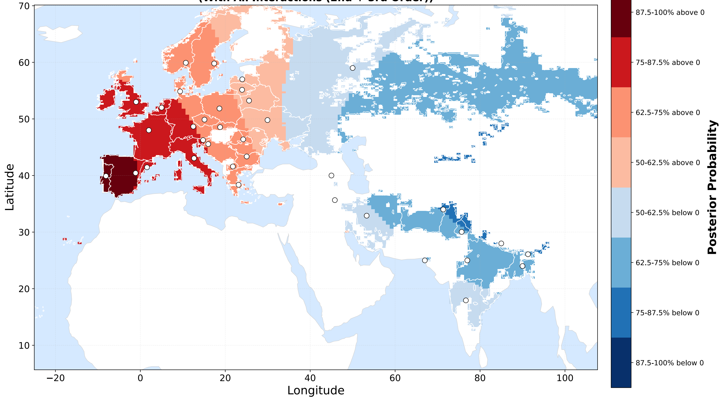
Posterior Probability of Positive Spline Effect: Speech (With All Interactions (2nd + 3rd Order))
