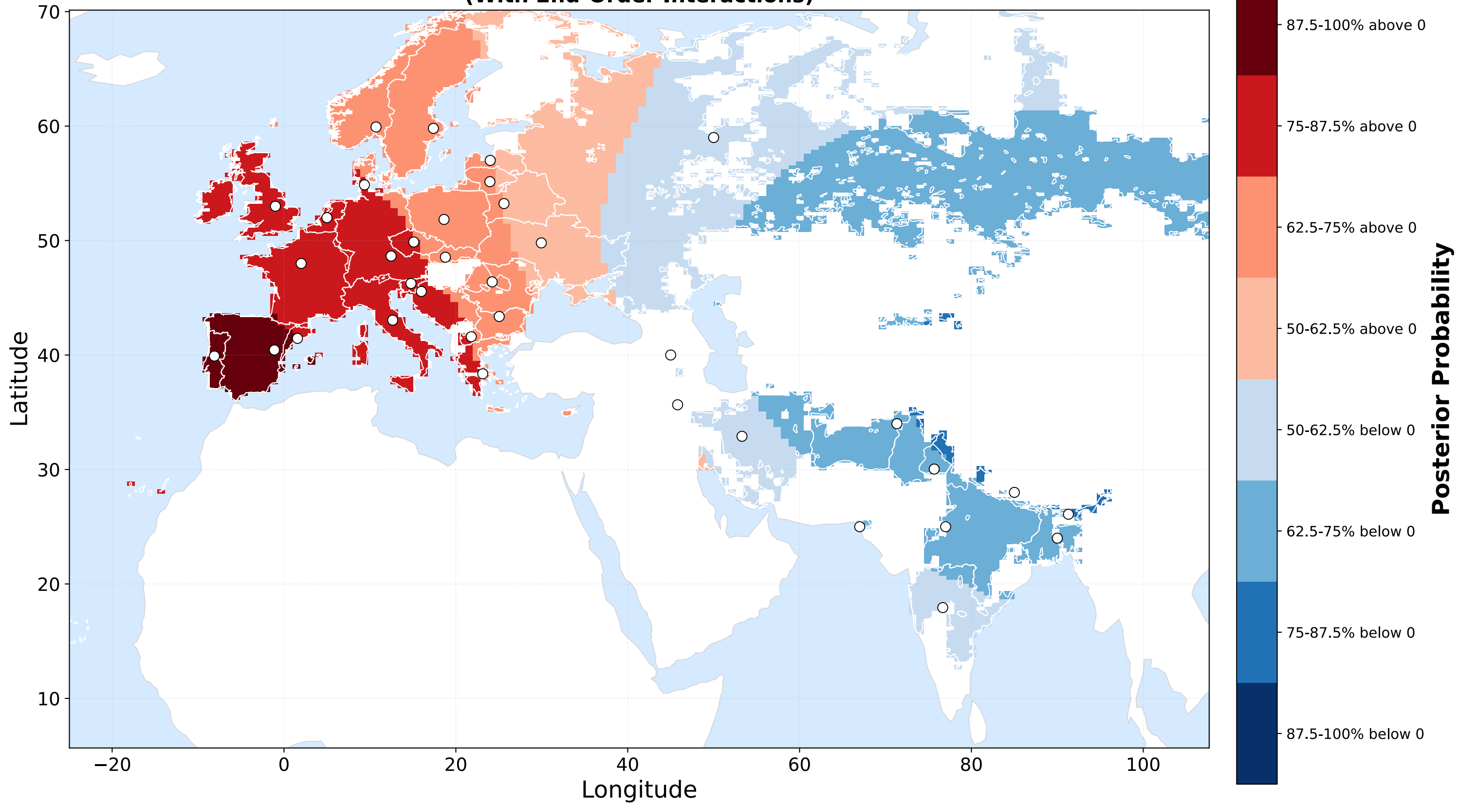
Posterior Probability of Positive Spline Effect: Speech (With 2nd-Order Interactions)
