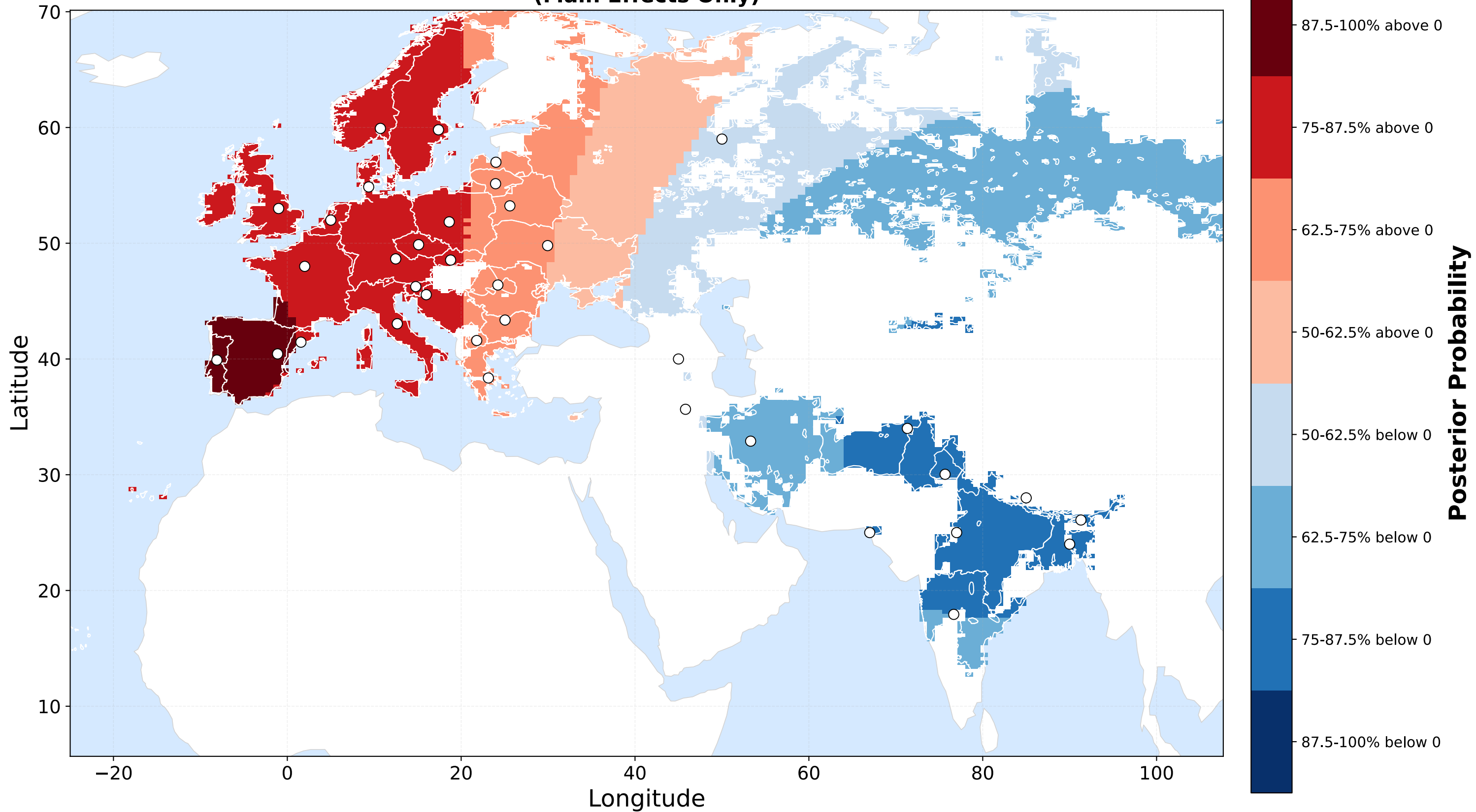
Posterior Probability of Positive Spline Effect: Speech (Main Effects Only)
