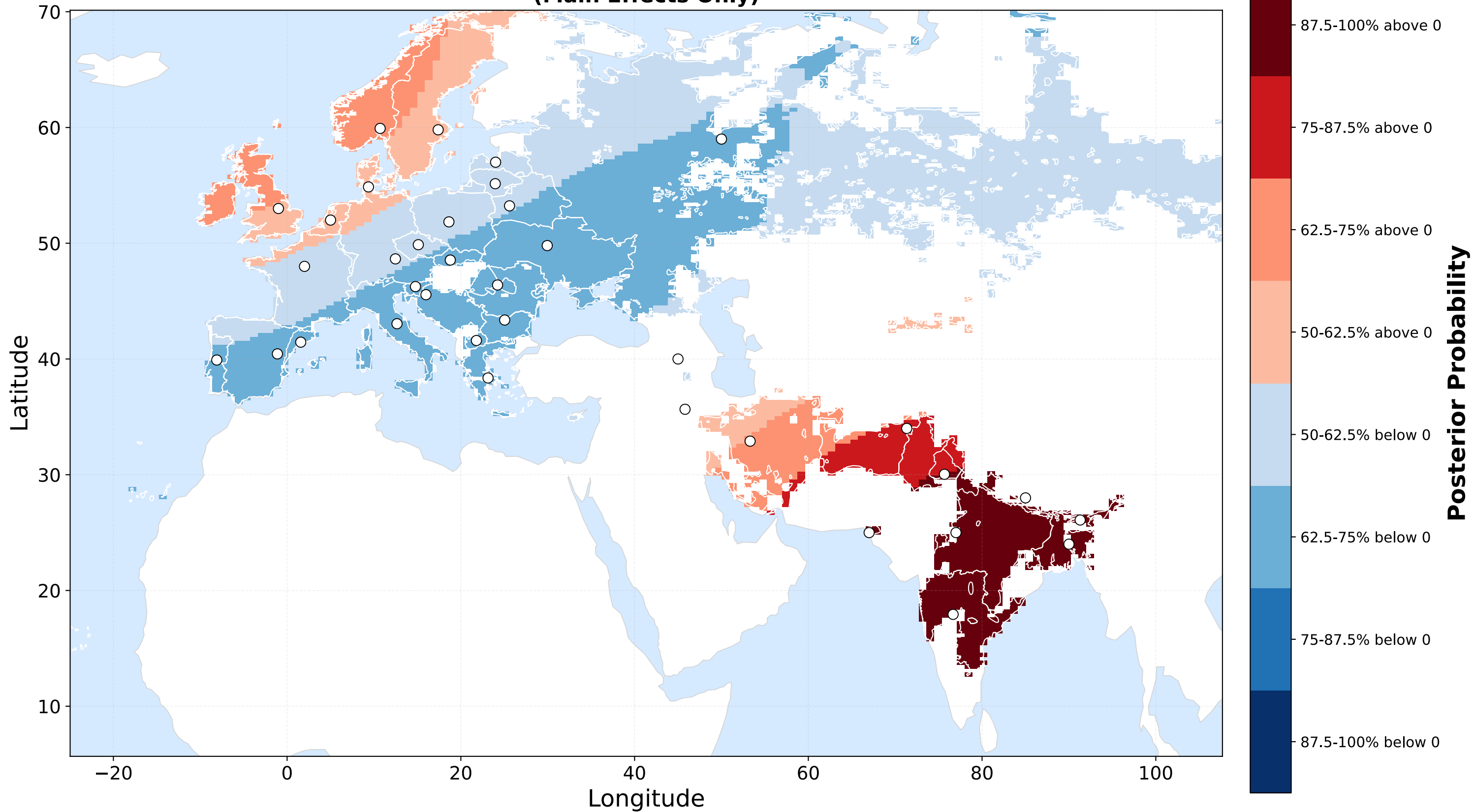
Posterior Probability of Positive Spline Effect: Cognates (Main Effects Only)
