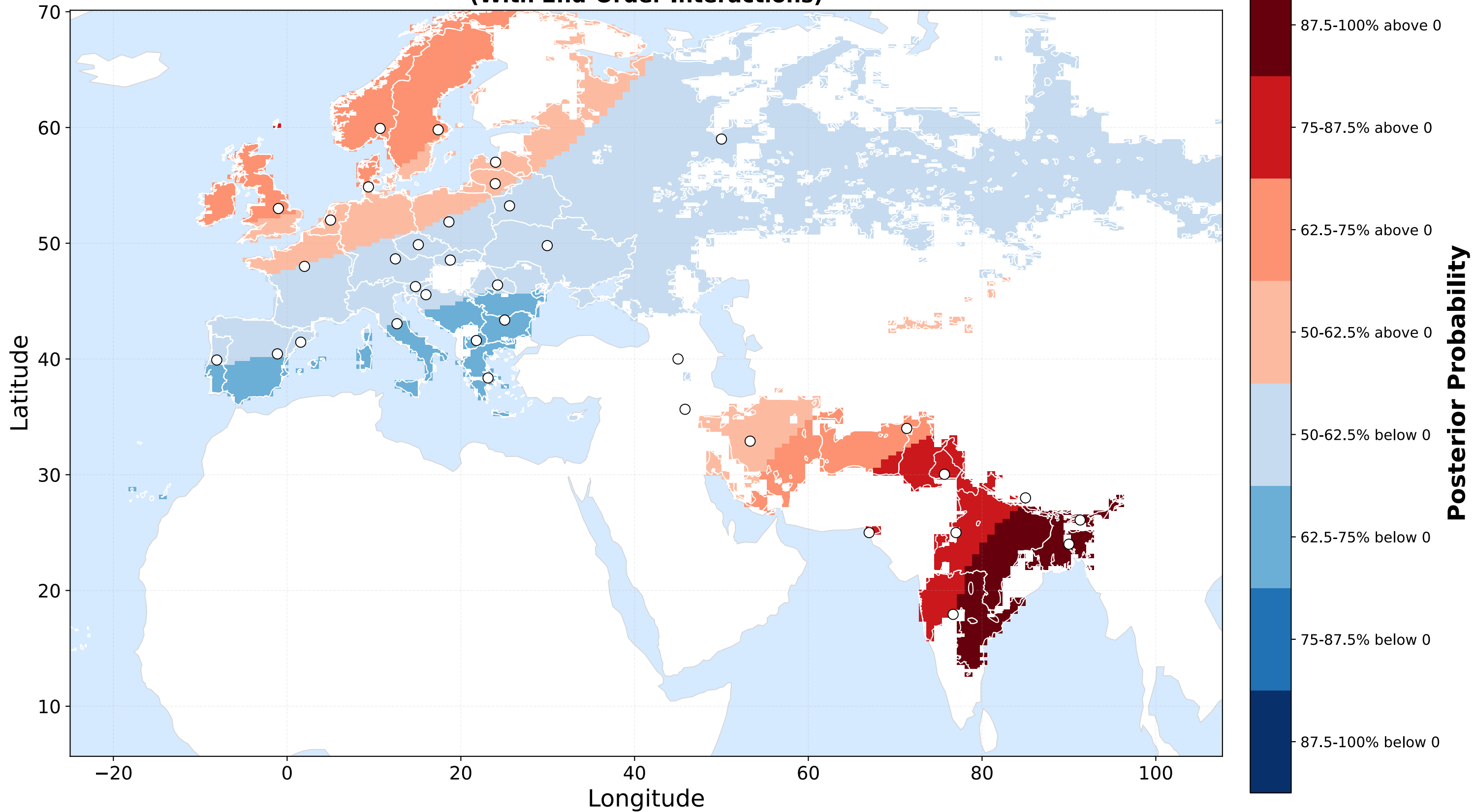
Posterior Probability of Positive Spline Effect: Cognates (With 2nd-Order Interactions)
