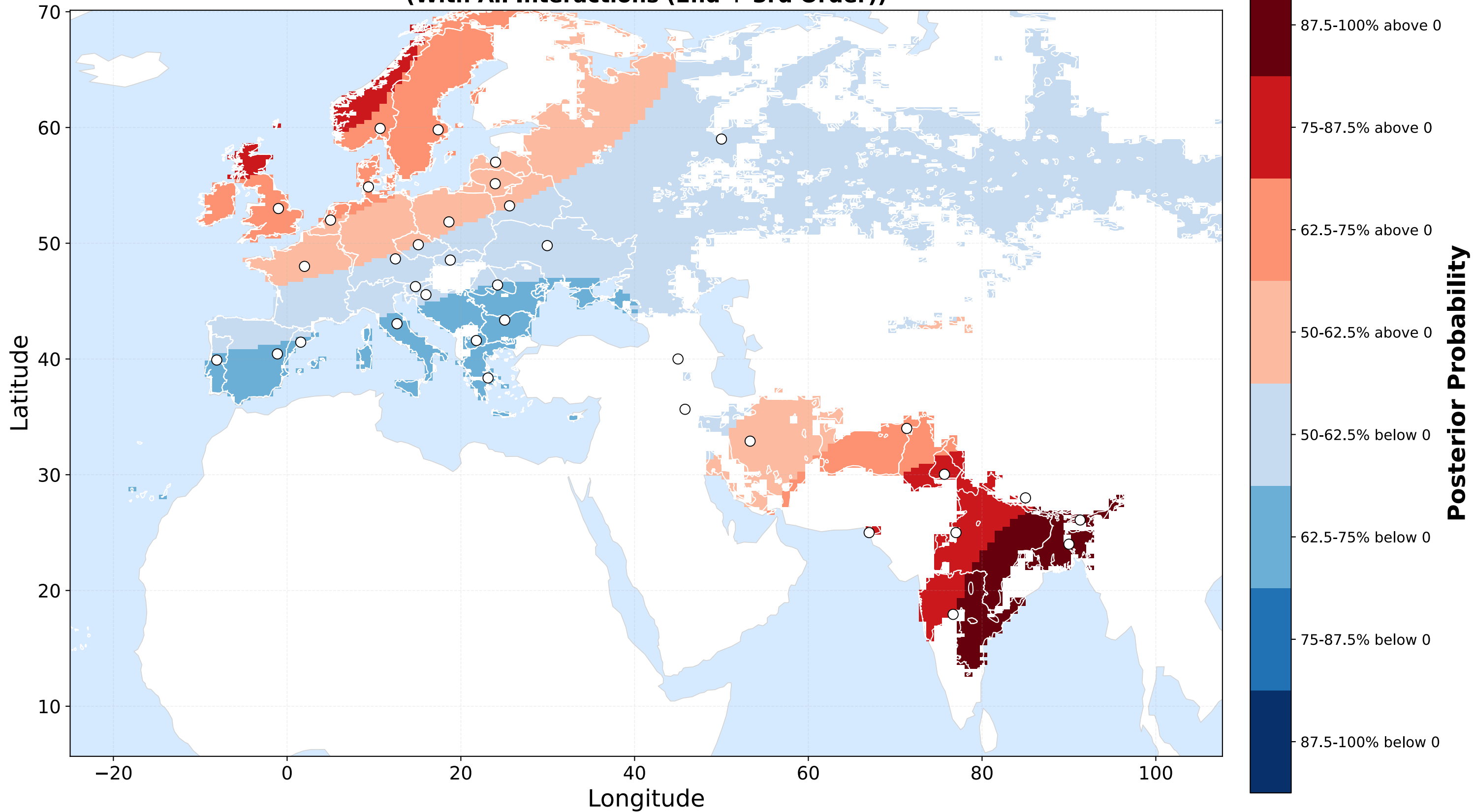
Posterior Probability of Positive Spline Effect: Cognates (With All Interactions (2nd + 3rd Order))
