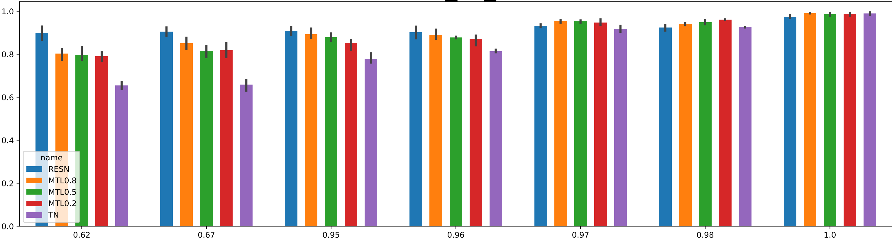
NIFO_ds_acc
