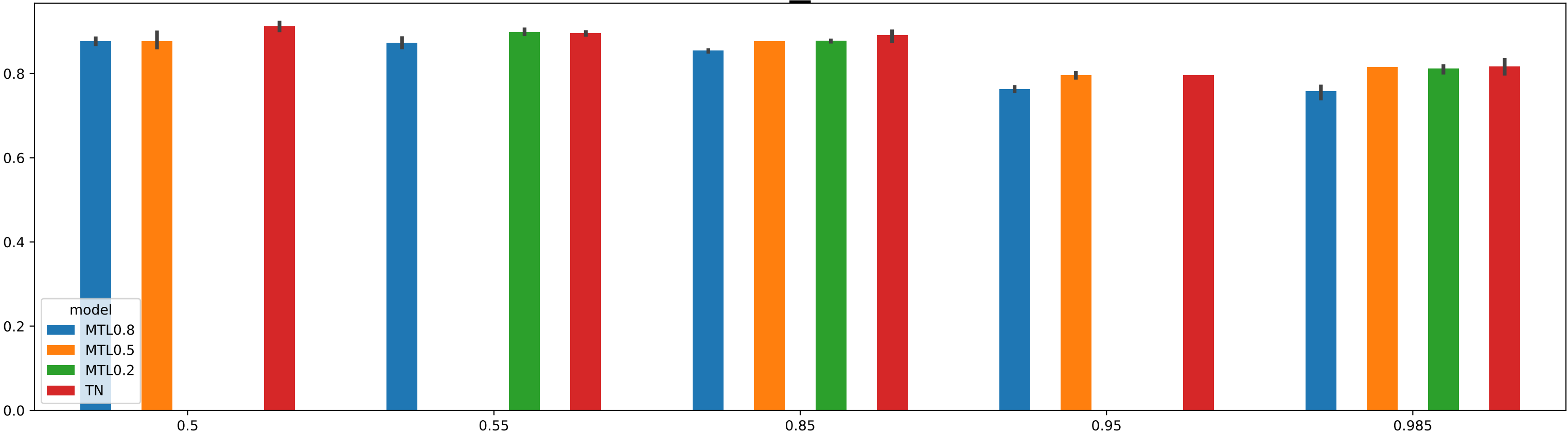
h2h_512
