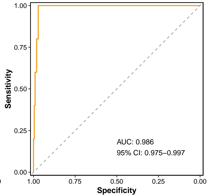
Dataset4---TCGA cohort
