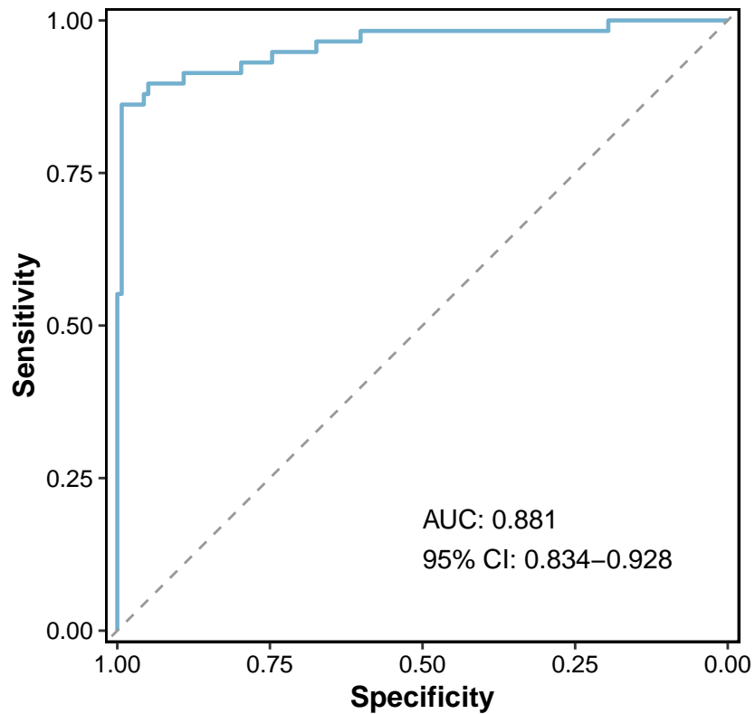
Dataset2---Internal Testing
