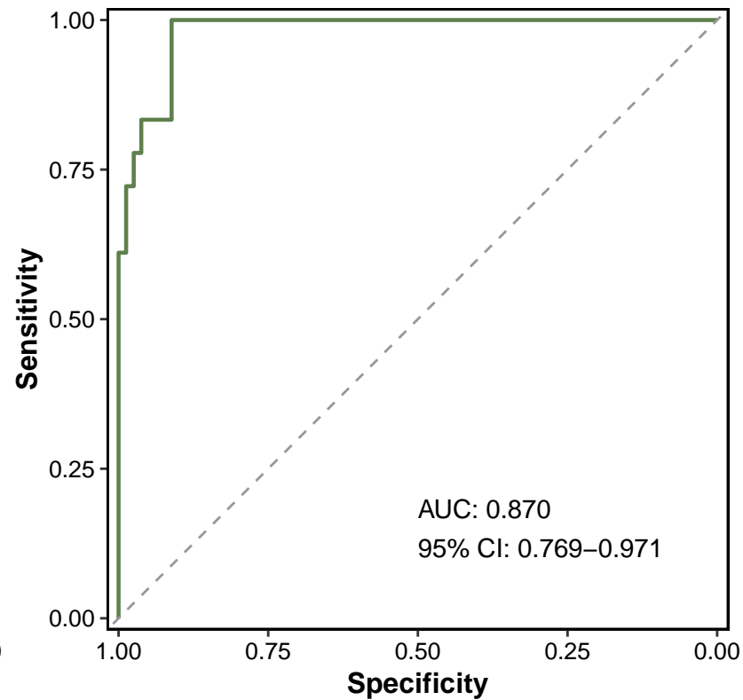
Dataset3---Multicenter
