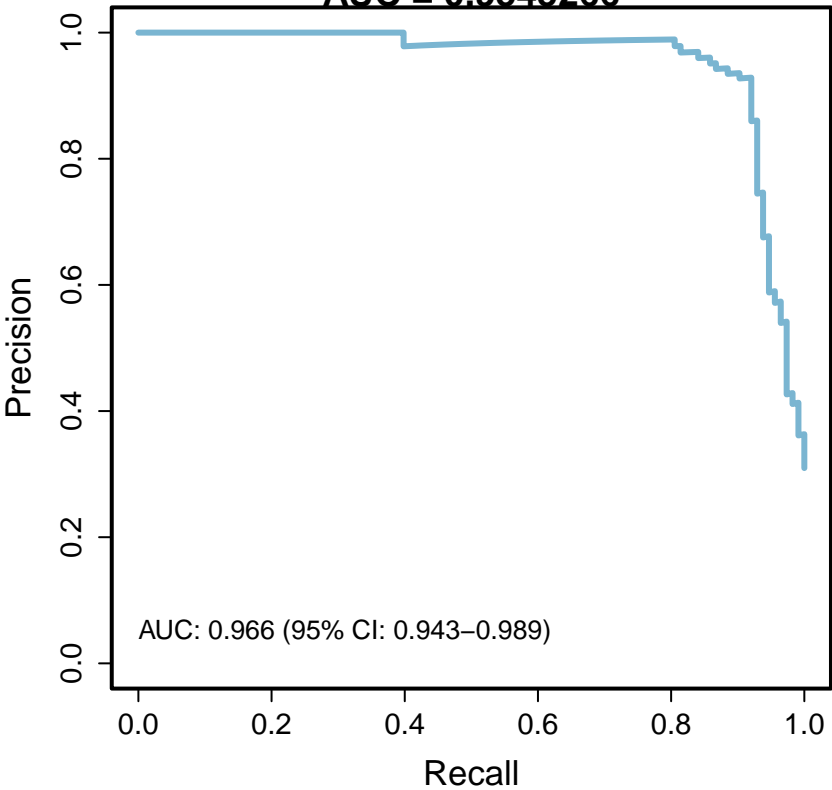
PR curve Recall Curve AUC = 0.9545266
