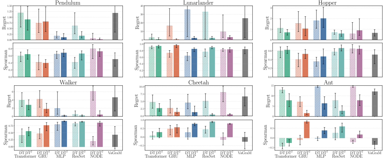
Figure 4. Regret and Spearman’s correlation for preference orderings from \mathcal{L}_{\text{sim}}^{\text{NLL}} (hashed) and \mathcal{L}_{\text{DT}^2} (solid) DTs across base architectures in six continuous control environments. Adapted VaGraM method shown in grey. We report averages over 10 seeds, with 95% CIs.
