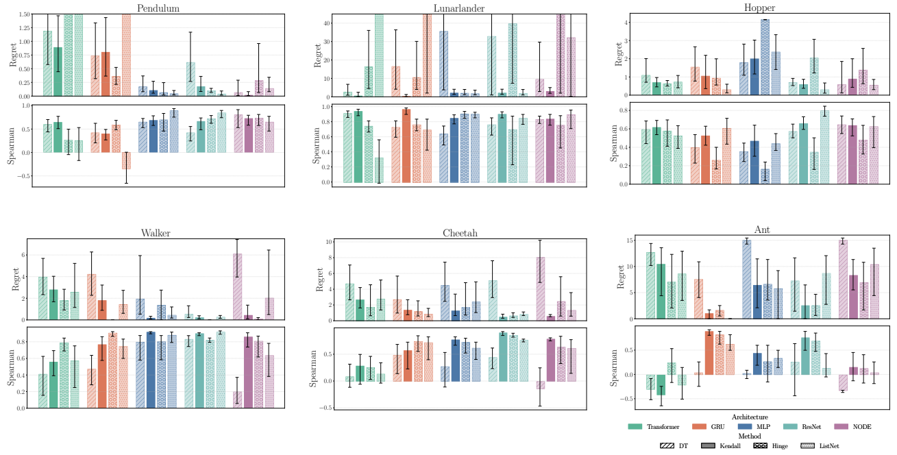
Figure 7. Regret and Spearman's correlation for preference orderings from \mathcal{L}_{sim}^{NLL} DTs (hashed), DT^2 using our smoothed Kendall's loss (solid), DT^2 using a hinge loss (circles), and with DT^2 using a ListNet loss (dotted) across different base architectures. We report averages over 10 seeds, with 95% CIs. For visual purposes, the top end of some bars are cropped out.
