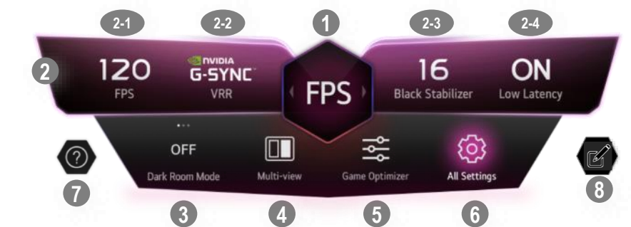
for Console game (HDMI Input)
