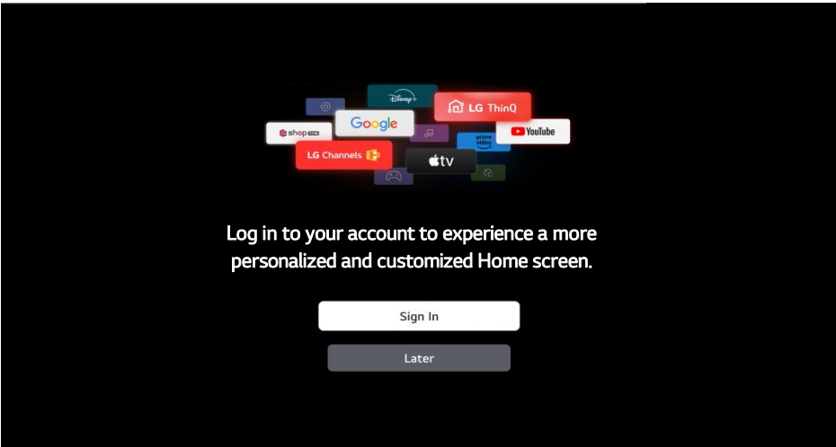
Account Guide
