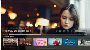
Interactive Dock
