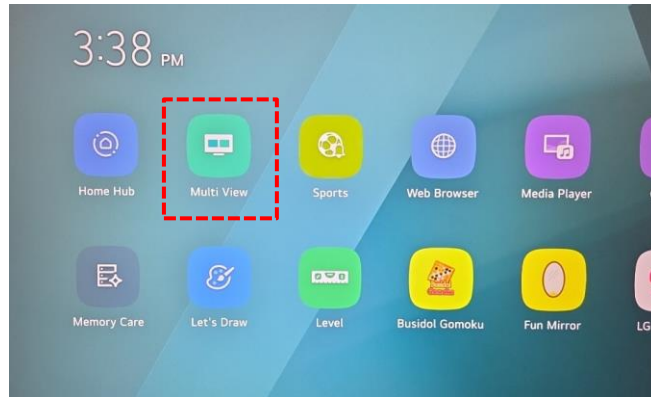
Multi View
