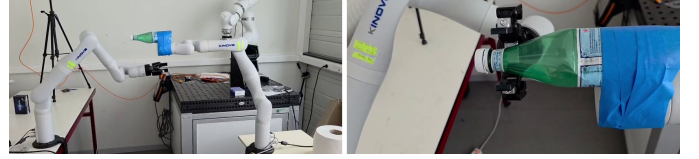
Fig. 11. The two physical arms in the laboratory, from the video record. Left: Robot B (right arm) presents the bottle while Robot A (left arm, Robotiq gripper) approaches. Right: Robot A's gripper closes around the bottle neck while Robot B still supports it.
