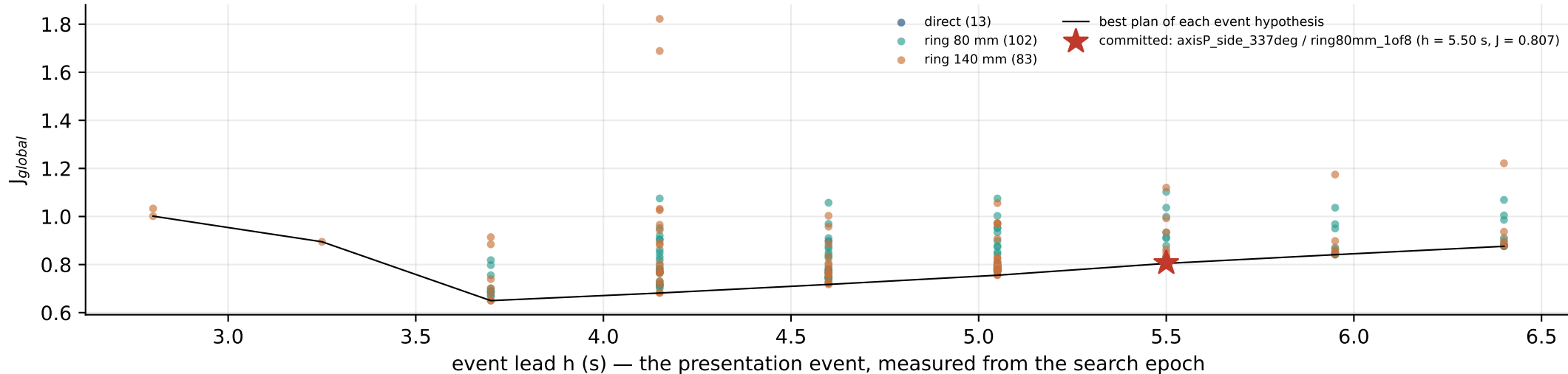
A every certified complete plan of «longitudinal»: 198 plans over 9 event hypotheses
