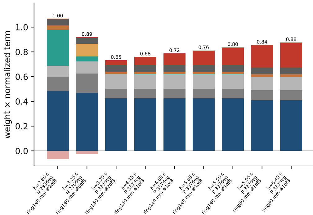
B best plan of each event hypothesis: which term moves with the event time
