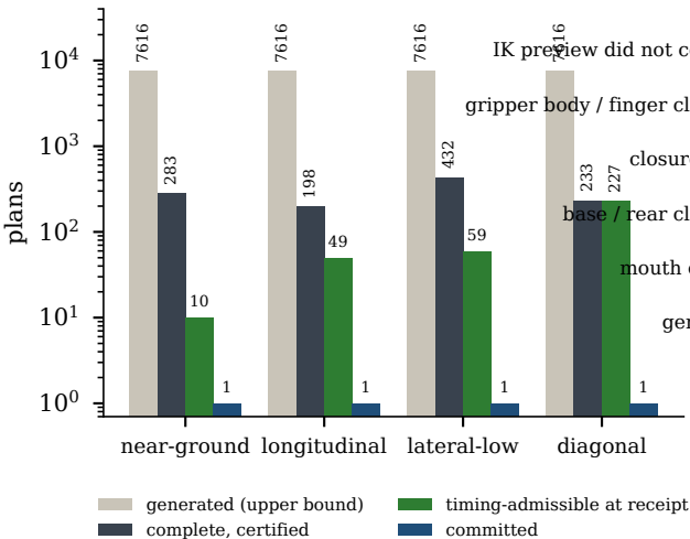
from the bank to one committed plan
