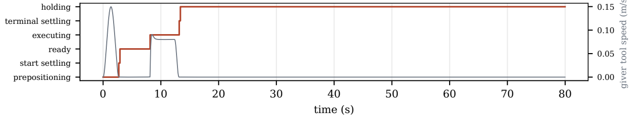
Robot B (giver): coordinator phase and tool speed
