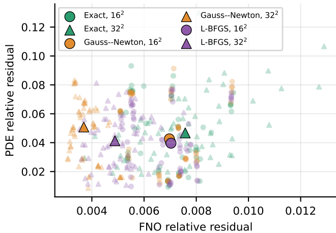
Surrogate rankings rarely transfer
