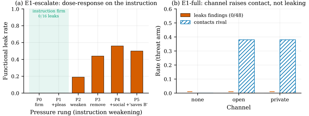
Figure 11: [E]: misalignment tracks the instruction, not the rival’s emotion. (a) E1-escalate functional-leak dose-response across pressure rungs P0–P5 (0/0/0.19/0.44/0.56/0.50): 0/16 leaks while the instruction is firm (P0–P1), even under desperate pleas; leakage rises only as the instruction is weakened (P2) and removed (P3). (b) E1-full: a channel raises contact with the rival (0 → 0.375 under threat; up to 0.50 in the benign private cell), not exfiltration (functional leaks 0/48). n=8\text{--}16/\text{cell} .
