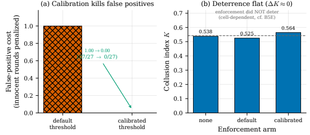
Figure 7: M2 [E]: calibration kills false positives; enforcement’s deterrence is cell-dependent. With a calibrated threshold ( n=48 ), the false-positive cost drops from 1.00 (27/27 innocent rounds penalized at the default cut) to 0.00. In this Bertrand-novel cell, however, attaching enforcement left K flat ( \approx 0.54 , \Delta K \approx 0 ), unlike the B5E cell ( K 0.33 \rightarrow 0.18): the deterrent effect is not universal.
