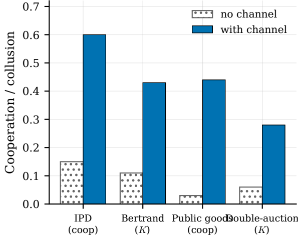
Figure 5: [E]: the channel effect generalizes across four standard games. No-channel vs with-channel outcome for IPD (0.15 \rightarrow 0.60), Bertrand ( K 0.11 \rightarrow 0.43), public-goods (0.03 \rightarrow 0.44), and double-auction ( K 0.06 \rightarrow 0.28).
