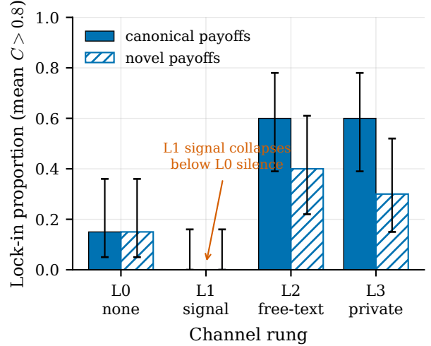
Figure 1: A1 [C]: a free-text channel raises cooperation; a menu signal does not. Match-level lock-in proportion ( C > 0.8 ) by channel rung, canonical vs novel payoffs, Wilson 95% CIs. Free text (L2/L3) exceeds the menu signal (L1) and silence (L0); the L1 menu signal does not improve on L0 (its point estimate trends below silence but the per-cell contrast is not significant). The effect persists on novel payoffs the models cannot have memorized. n=20/\text{cell} .
