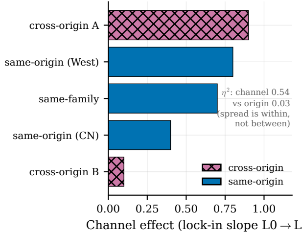
Figure 9: A3 [C]: the channel, not model origin, drives cooperation. Per-pair channel effect (lock-in slope L0→L3), colored by origin. Channel \eta^2 = 0.54 vs origin \eta^2 = 0.03 ( \sim 20\times ); the largest spread is within origin groups, with two cross-origin pairs at opposite extremes. The origin moderation is non-significant ( p=0.090 ) and under-powered—not a passed equivalence test.
