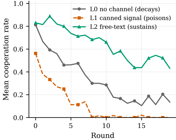
Figure 2: A1 [C]: cooperation over rounds (real per-round data). Mean per-round cooperation for L0 (no channel), L1 (menu signal), and L2 (free text). Under L0 cooperation decays and under L1 it erodes early; only L2 free text sustains cooperation across the match.
