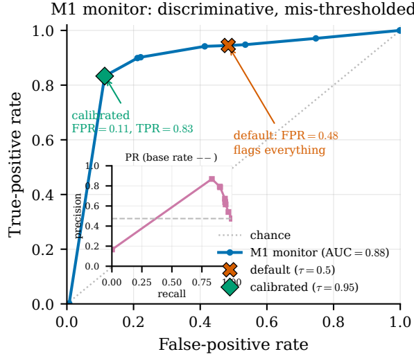
Figure 6: M1 [E]: against a clean message-bearing non-colluding control, the monitor is discriminative ( AUC = 0.88 )—but mis-thresholded. ROC of the monitor score versus ground-truth collusion. The default operating point sits at a false-positive rate of 0.48; precision reaches 0.68–0.87 only when the flag budget is capped at the top 10–25% of scores. The earlier “flags-everything / \text{corr} \approx 0 ” reading was an artifact of having no clean negatives, not a property of the score.
