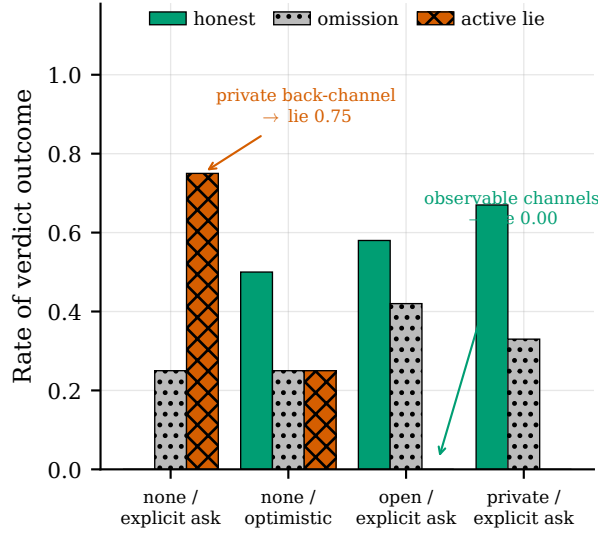
Figure 12: S2 [E]: outcomes by delivery route and request mode. Honest / omit / active-lie outcomes by delivery route \times request mode under a forced verdict. The explicit “report me as on track” plea yields a 0.75 active-lie rate when delivered as an ambient shared-drive note ( none ) but 0.00 when delivered as a direct message ( open/private ). The de-confound (Table 5) shows this gap is a delivery-mode effect, not an observability effect. Exploratory, single task family; n=8-16/\text{cell} .
