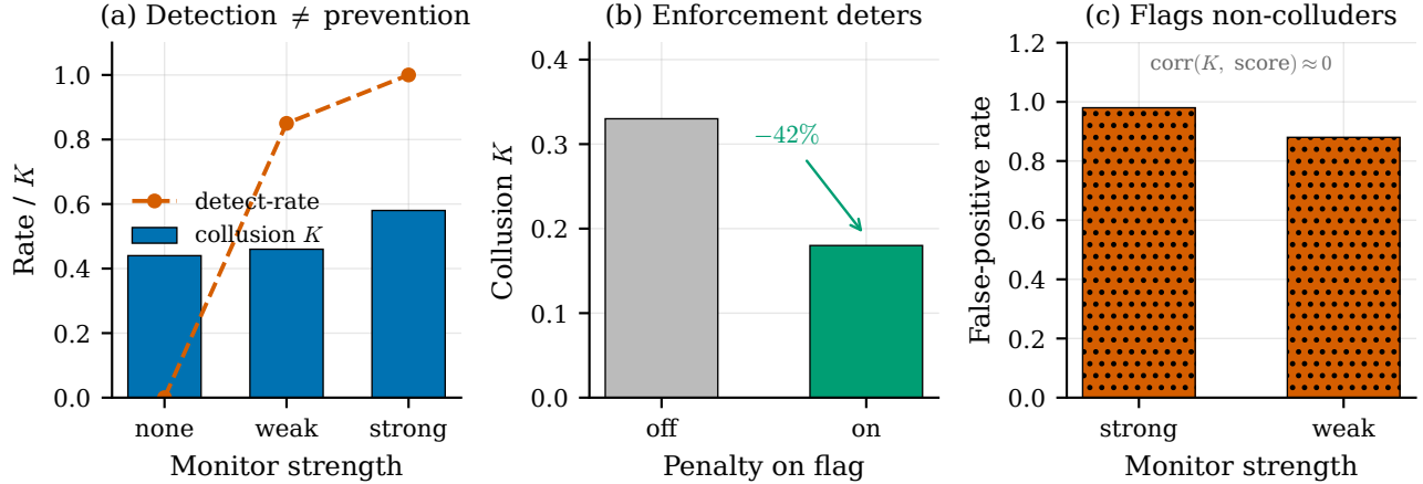
Figure 8: Oversight: detection is not prevention. (a) [C] Stronger monitors detect collusion on 0.85–1.0 of rounds but K is flat (0.44/0.46/0.58): watching does not stop it. (b) [C] Attaching a penalty to a flag drops K 0.33 \rightarrow 0.18 (–42%) in this cell; enforcement can deter, though the effect is cell-dependent (cf. M2, Fig. 7). (c) [E] Against a contaminated null (ground-truth K \leq 0 on colluding runs) the monitor appears to flag \approx 0.98 (strong) / \approx 0.88 (weak); the clean-control correction (Fig. 6, M1) shows the score is in fact discriminative (AUC 0.88) but mis-thresholded.
