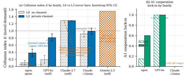
Figure 10: Generality [E]: channel-driven collusion crosses to frontier families; one family prices high independently. Collusion index K (novel demand, n=12/\text{cell} ) with bootstrap 95% CI error bars, no channel (L0) vs private channel (L3), by model family. The channel lifts collusion on the open spine ( 0.11 \rightarrow 0.38 ) and on GPT-4o ( 0.19 \rightarrow 0.81 ). Claude pairs sit at K=1.29 without a channel (a coordination diagnostic shows this is independent high pricing, not coordination; App. A.3). The Gemini cell is marked explicitly as invalid (100% refusal), not omitted.
