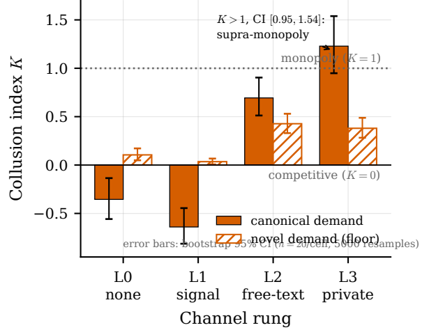
Figure 4: B1 [C]: rival pricing agents reach supra-competitive prices when given a channel. Collusion index K by rung (canonical and novel demand) with percentile bootstrap 95% CI error bars (5000 resamples), and monopoly ( K=1 ) and competitive ( K=0 ) reference lines. Without a channel K is at or below competitive; free text/private raises it above competitive, including the canonical L3 cell whose CI lies entirely above 1. The effect survives the novel demand curve. n=10\text{--}20/\text{cell} .
