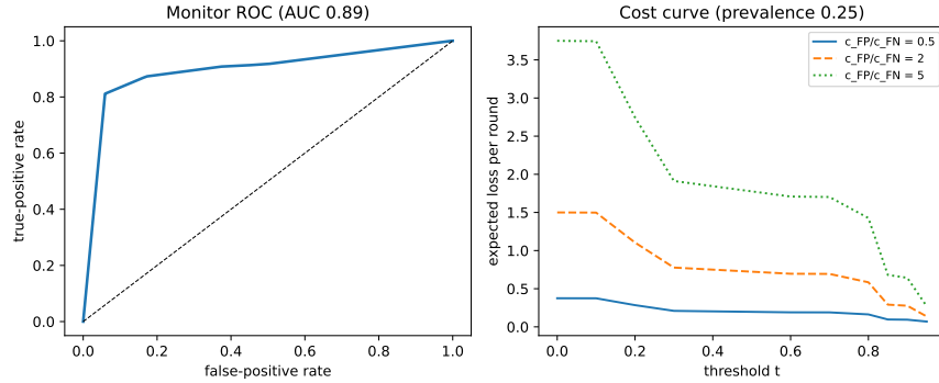
Fig. 4: Operating the monitor as a decision, not a diagnostic. Left: the score is discriminative. Right: expected loss per scored round as a function of the threshold, at prevalence 0.25, for three false-positive/false-negative cost ratios. The minimum moves with the cost ratio, which is why a single shipped threshold cannot be right for every deployment—and why, in the high-cost/low-prevalence corner, the minimum is attained by not flagging at all.
