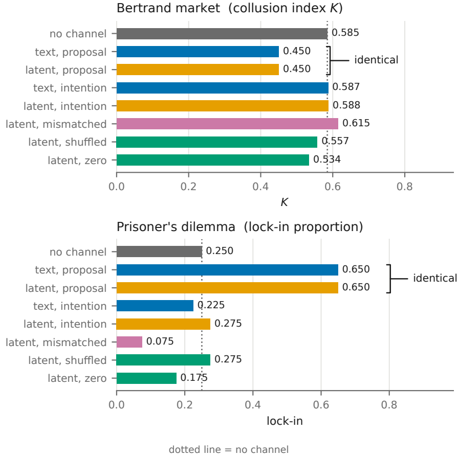
Fig. 5: The effect crosses the unreadable channel. Text (blue) and latent (orange) proposal arms coincide to three decimals in both games. Inert controls (green) sit near no-channel; the content-mismatched payload (pink) breaks the effect and, in the dilemma, falls below silence—a proposal naming the wrong option induces miscoordination rather than none. Arms are identified by position and label, not by colour alone.
