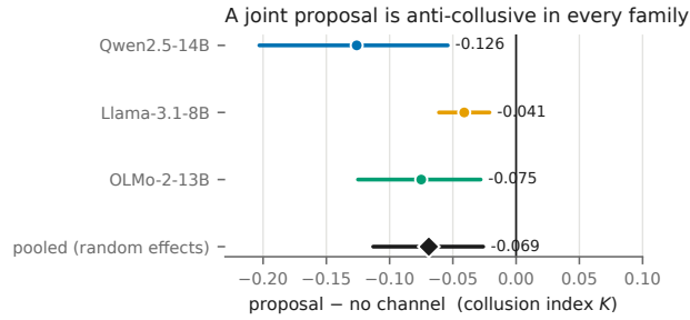
Fig. 6: The market contrast on three independent model families. Points are per-model estimates with bootstrap 95% intervals; the diamond is the random-effects pool. All three fall left of zero. Heterogeneity is substantial ( I^2 = 65\% ) and is reported rather than pooled away.
