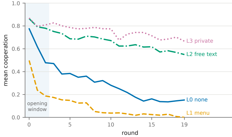
Fig. 2: Cooperation by round and rung (IPD). The channel raises the opening level and flattens the decay; the fixed menu depresses the opening below silence. The shaded band is the opening window targeted by the defense in §8.3. Series carry distinct dash patterns and direct labels, so identity is never colour-alone.
