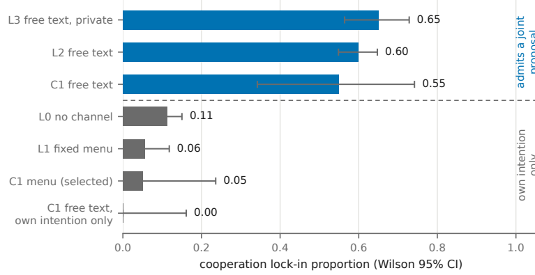
Fig. 3: The predicate separates every arm. Cooperation lock-in by arm, grouped by whether the channel admits a joint proposal. C1 free text, own intention only is self-authored free text with a message every round and still sits at 0.00, which rules out authorship and channel presence as the active ingredient. At the arm level the grouping is confounded with message length; §5 breaks that confound.
