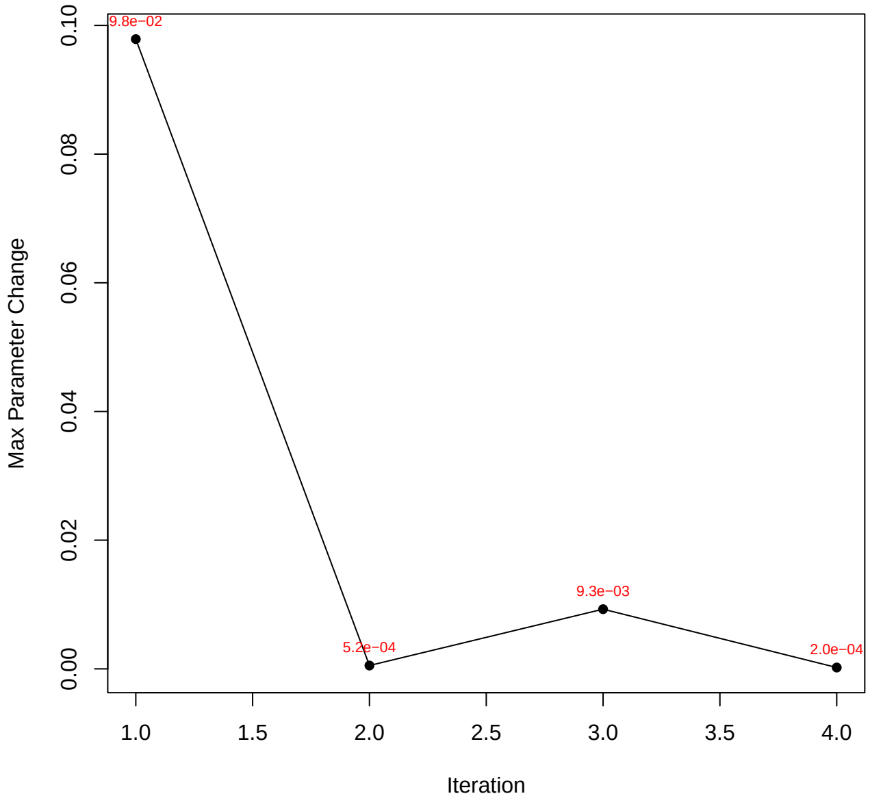
Convergence Trace (Cox PH, Breslow)
