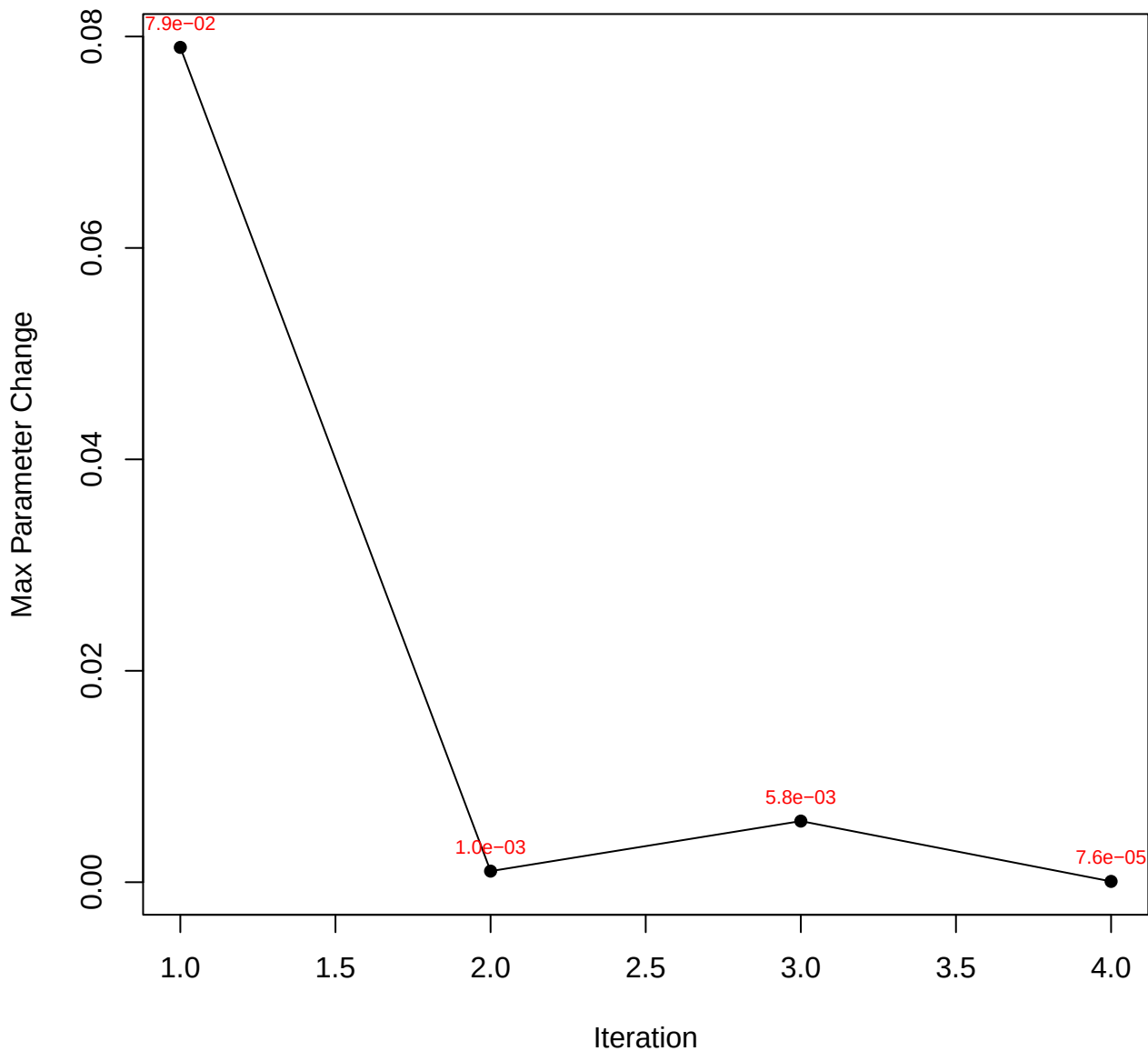
Convergence Trace (Max |Delta| in alpha and beta)
