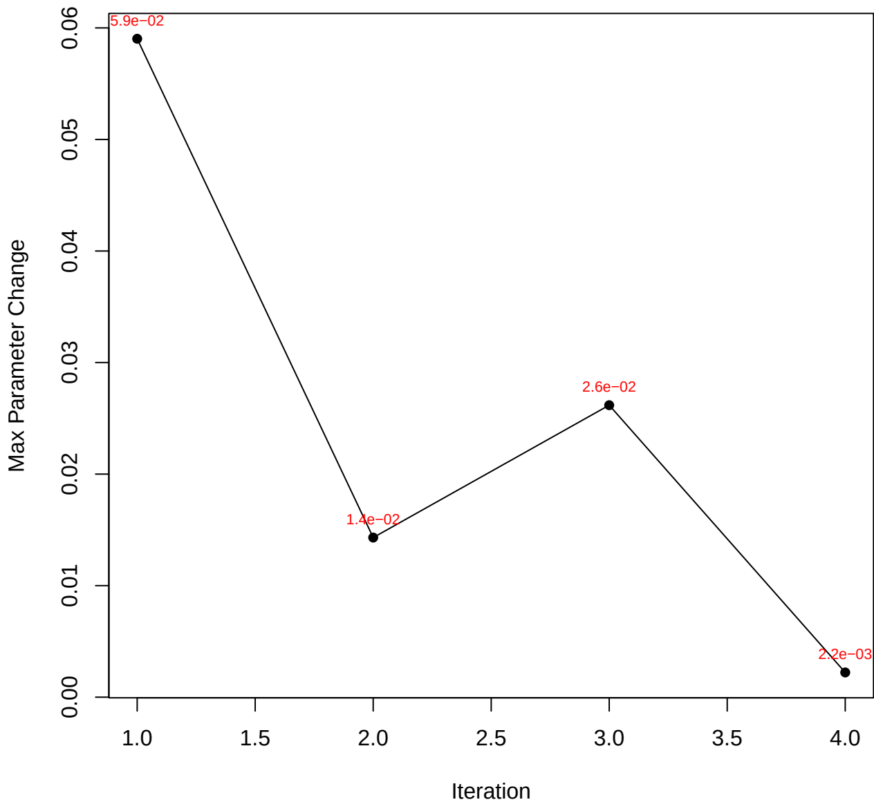
Convergence Trace (mgcv ocat)
