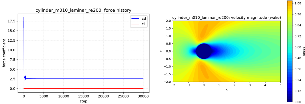
Figure 4: Cylinder Re200: force history (cl stays flat — no shedding develops at this resolution) and velocity-magnitude wake.
