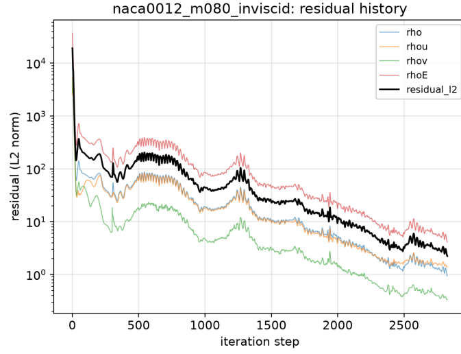
Figure 8: NACA0012 inviscid, M_\infty = 0.80 : residual history (per-equation L2 and global L2).
