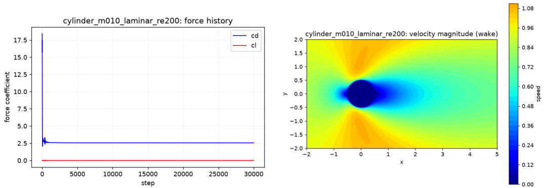
Figure 4: Cylinder Re200: force history (cl stays flat with the default Rusanov flux; the AUSM + -up flux excites shedding (cl 0.07–0.22) but it cannot be sustained past t \sim 10 due to mesh-resolution limits) and velocity-magnitude wake.
