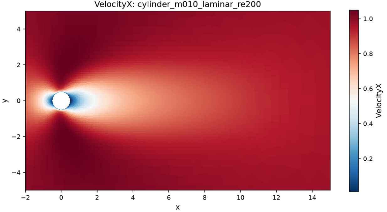
Figure 13: Velocity- x contour (wake region): cylinder, Re 200 vortex street.
