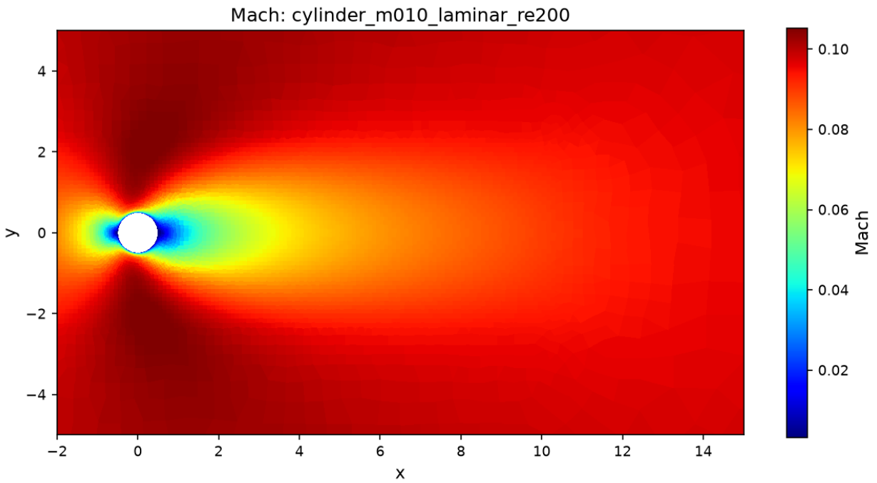
Figure 12: Mach contour (wake region): cylinder, Re 200 vortex street.
