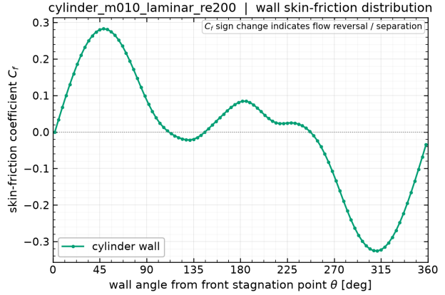
(f) Wall C_f at t = 300 .
