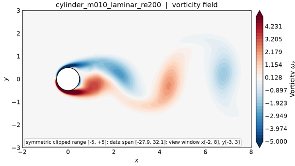
(a) Vorticity, clipped to [-5, 5] .
