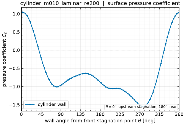
(e) Wall C_p at t = 300 .
