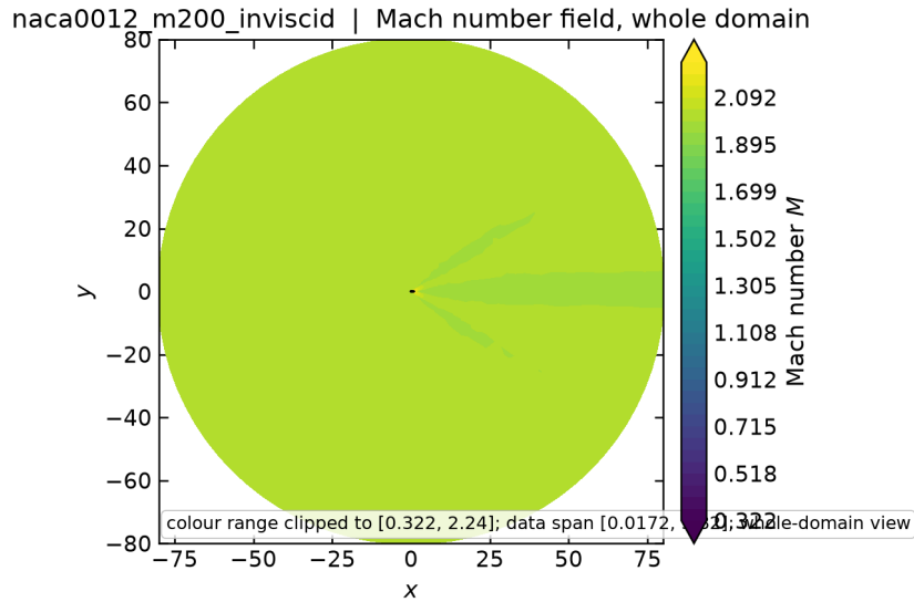
Figure 7: NACA0012 at M_\infty = 2.0 , inviscid: whole-domain Mach number from field_final.vtu . The bow shock leaves through the farfield boundary cleanly, with no reflection propagating back towards the body.
