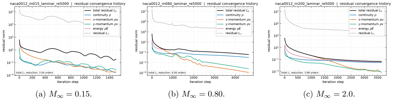
Figure 11: Residual histories for the three laminar NACA0012 cases at Re = 5000 , from each residuals.csv .
