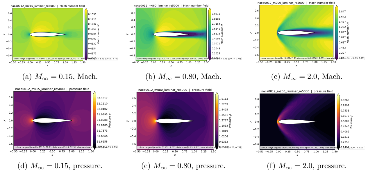
Figure 14: Laminar NACA0012 cases at Re = 5000 : near-body Mach number (top) and pressure (bottom) from each field.final.vtu . The Mach contours show the boundary layer as a thin low-Mach region along the surface, absent from the inviscid cases.
