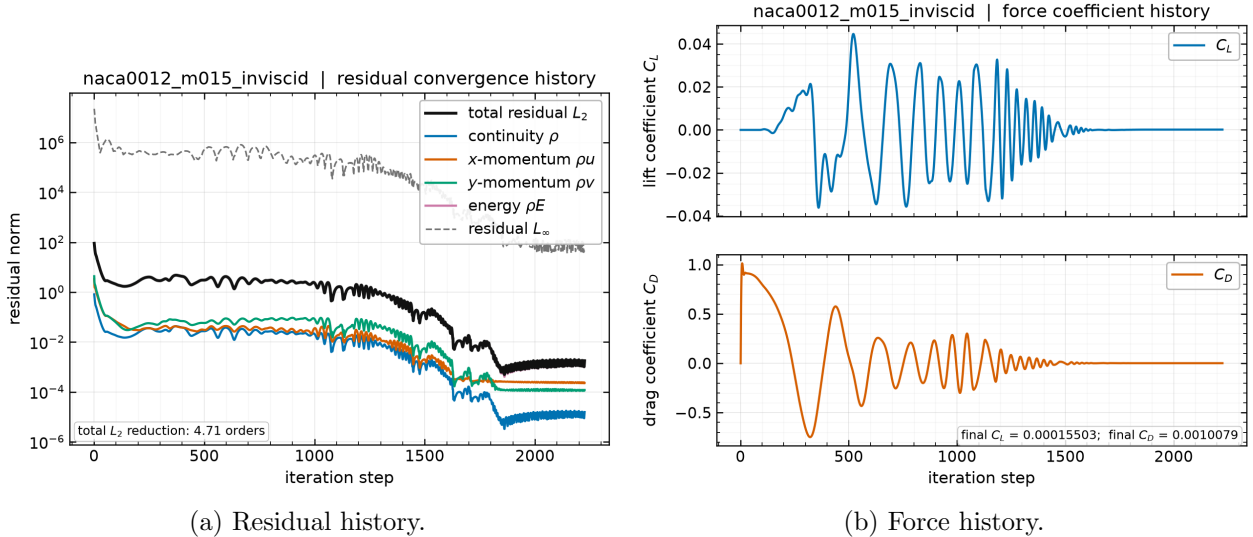
Figure 1: NACA0012 at M_\infty = 0.15 , inviscid. Left: total and per-component L_2 residual norms and the L_\infty norm against pseudo-time step, from residuals.csv . Right: C_L and C_D against step, from forces.csv .
