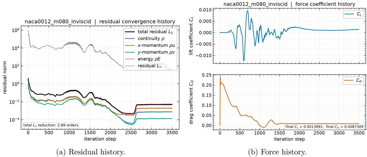
Figure 4: NACA0012 at M_\infty = 0.80 , inviscid: residual and force histories from residuals.csv and forces.csv .
