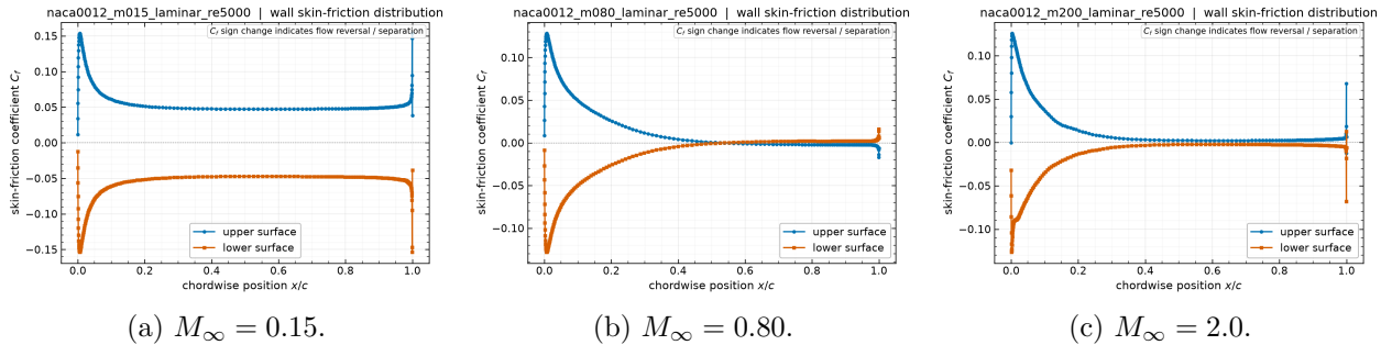
Figure 12: Skin-friction coefficient along the airfoil for the laminar cases, from the cf column of each surface.csv . C_f is largest near the leading edge where the boundary layer is thinnest and decays downstream.
