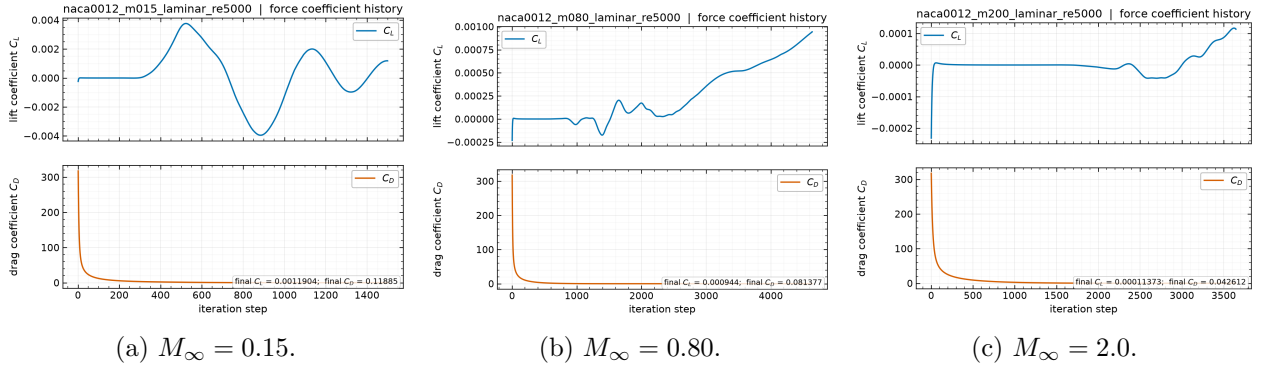
Figure 11: Force histories for the three laminar NACA0012 cases at Re = 5000 , from each forces.csv . These histories, not the residual norms, are the binding convergence evidence discussed in section 8.5.
