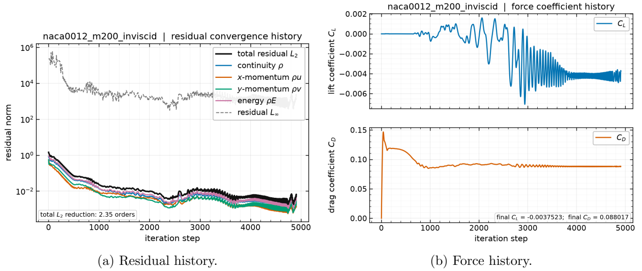
Figure 7: NACA0012 at M_\infty = 2.0 , inviscid: residual and force histories from residuals.csv and forces.csv .
