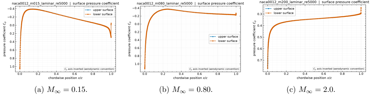
Figure 13: Surface pressure coefficient along the airfoil for the laminar cases at Re = 5000 , from the cp column of each surface.csv . Comparing these with the inviscid distributions of figs. 3, 6 and 9 isolates the effect of the boundary layer on the pressure field, which is largest near the trailing edge where the displacement thickness is greatest.
