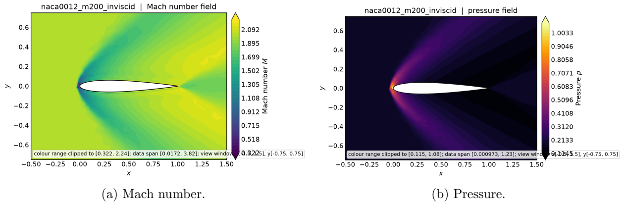
Figure 8: NACA0012 at M_\infty = 2.0 , inviscid: Mach and pressure contours from field_final.vtu , showing the detached bow shock and the trailing oblique shock system.
