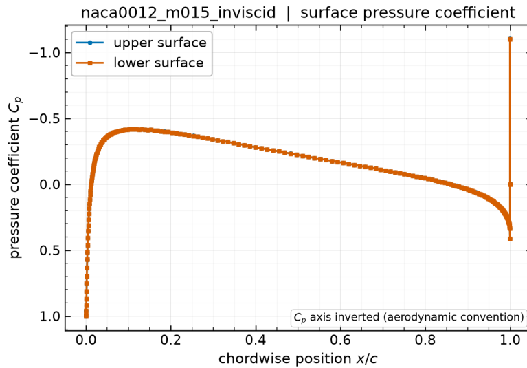
Figure 3: NACA0012 at M_\infty = 0.15 , inviscid: surface pressure coefficient against chordwise position from surface.csv . Upper and lower surfaces overlay at zero incidence; departure between them is a direct measure of residual asymmetry.
