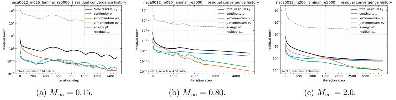
Figure 10: Residual histories for the three laminar NACA0012 cases at Re = 5000 , from each residuals.csv .
