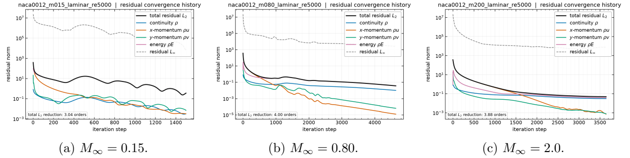
Figure 10: Residual histories for the three laminar NACA0012 cases at Re = 5000 , from each residuals.csv .
