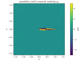
(f) vorticity field (from field_final.vtu).
