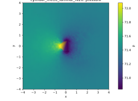
(f) pressure field (from field_final.vtu).
