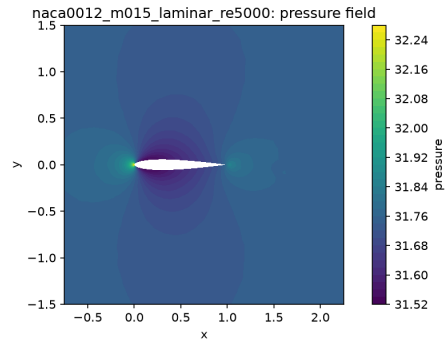
(e) Static-pressure field from field_final.vtu .
