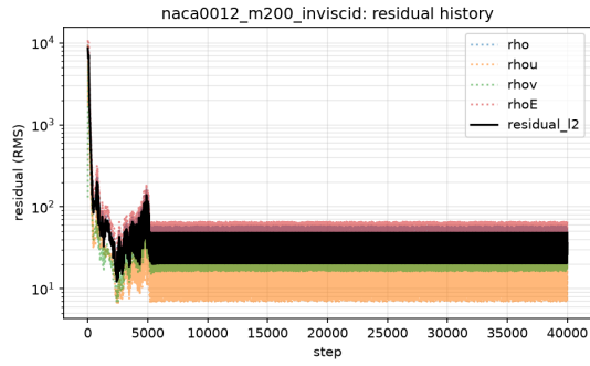
(a) Residual history from residuals.csv .
