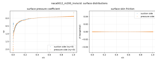
(c) Surface C_p from surface.csv .
