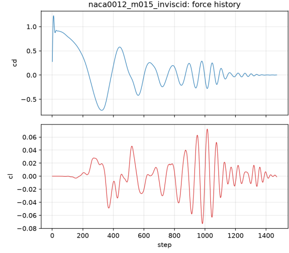
(b) Force-coefficient history ( C_D , C_L ) from forces.csv .
