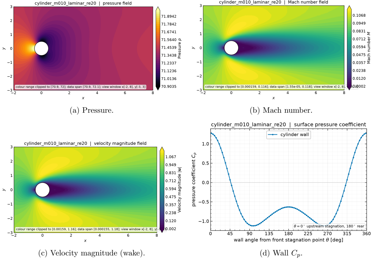
Figure 17: Cylinder at Re = 20 : fields from field_final.vtu and the wall pressure coefficient from surface.csv . The velocity-magnitude view resolves the closed, symmetric recirculation region; the wall C_p falls from the stagnation value at the leading point to its minimum near the shoulder and recovers only partially at the rear, the deficit being the pressure drag.
