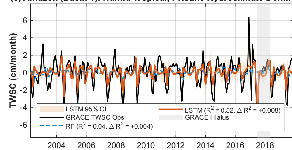
(c) Amazon (Basin 1): Humid Tropical, Pristine Hydroclimate Dominance
