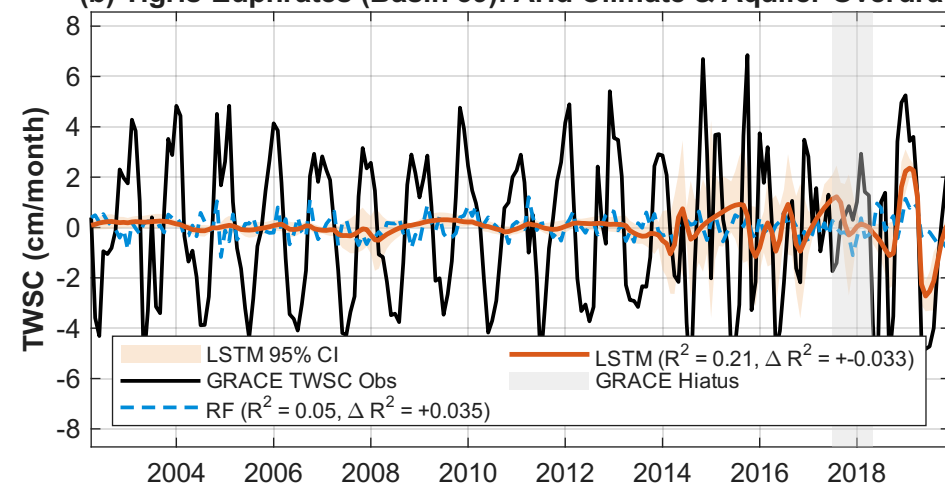
(b) Tigris-Euphrates (Basin 39): Arid Climate & Aquifer Overdraft
