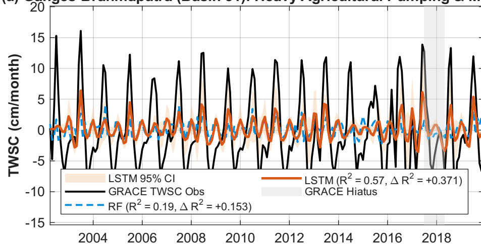
(a) Ganges-Brahmaputra (Basin 51): Heavy Agricultural Pumping & Monsoon
