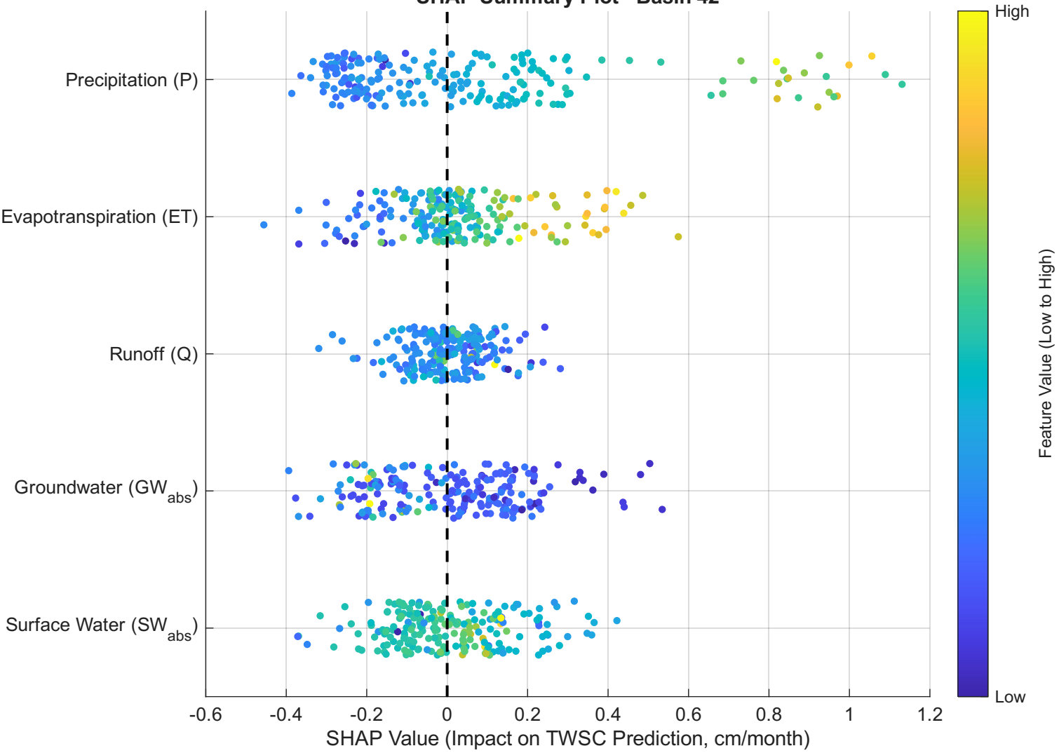
SHAP Summary Plot - Basin 42
