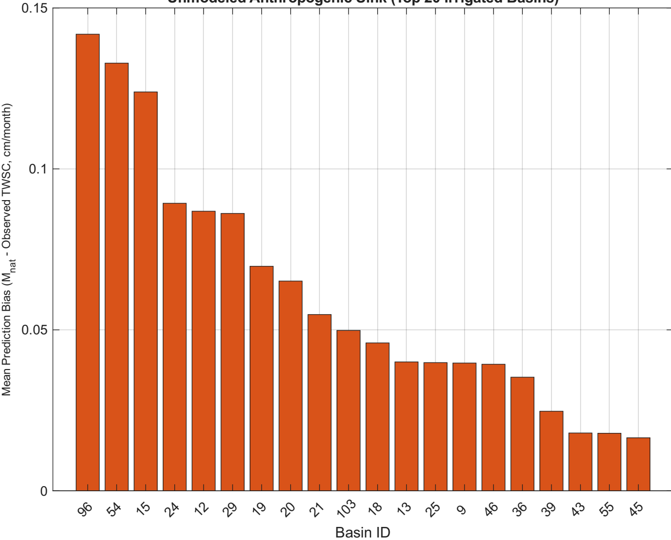
Unmodeled Anthropogenic Sink (Top 20 Irrigated Basins)
