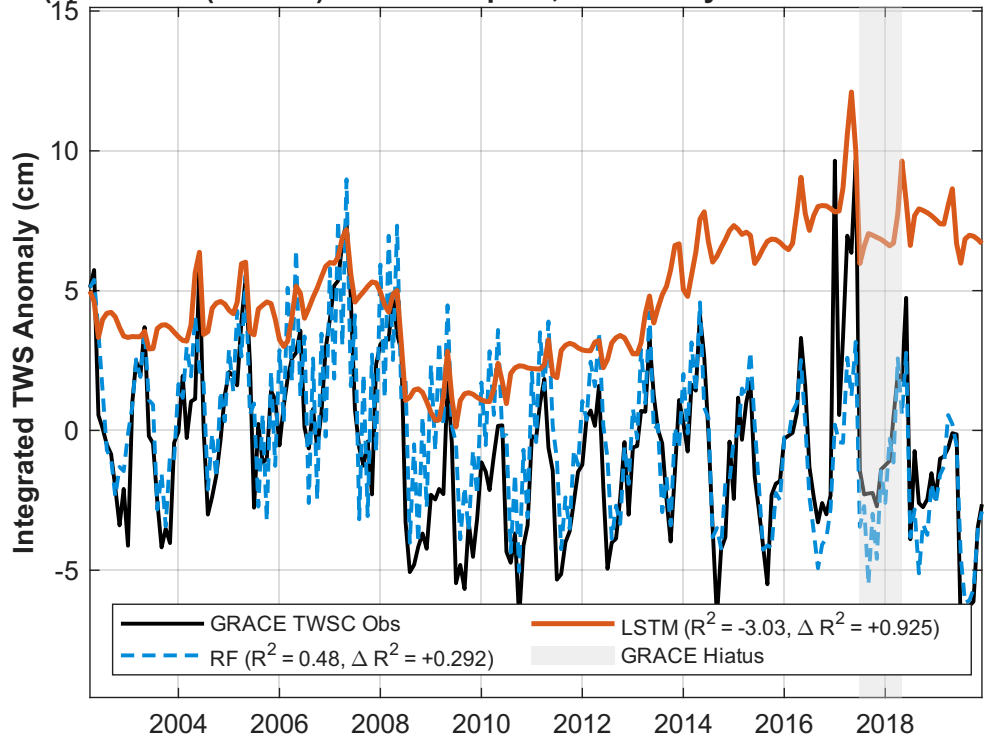
(c) Amazon (Basin 1): Humid Tropical, Pristine Hydroclimate Dominance
