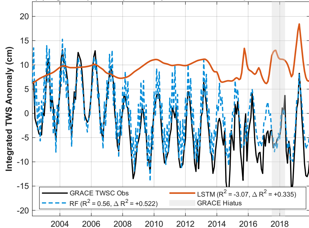
(b) Tigris-Euphrates (Basin 39): Arid Climate & Aquifer Overdraft
