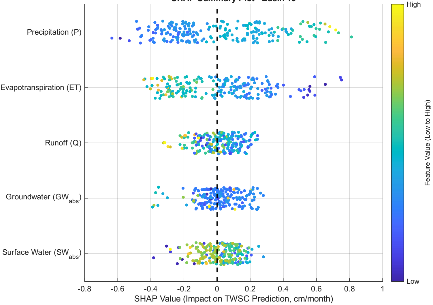
SHAP Summary Plot - Basin 13
