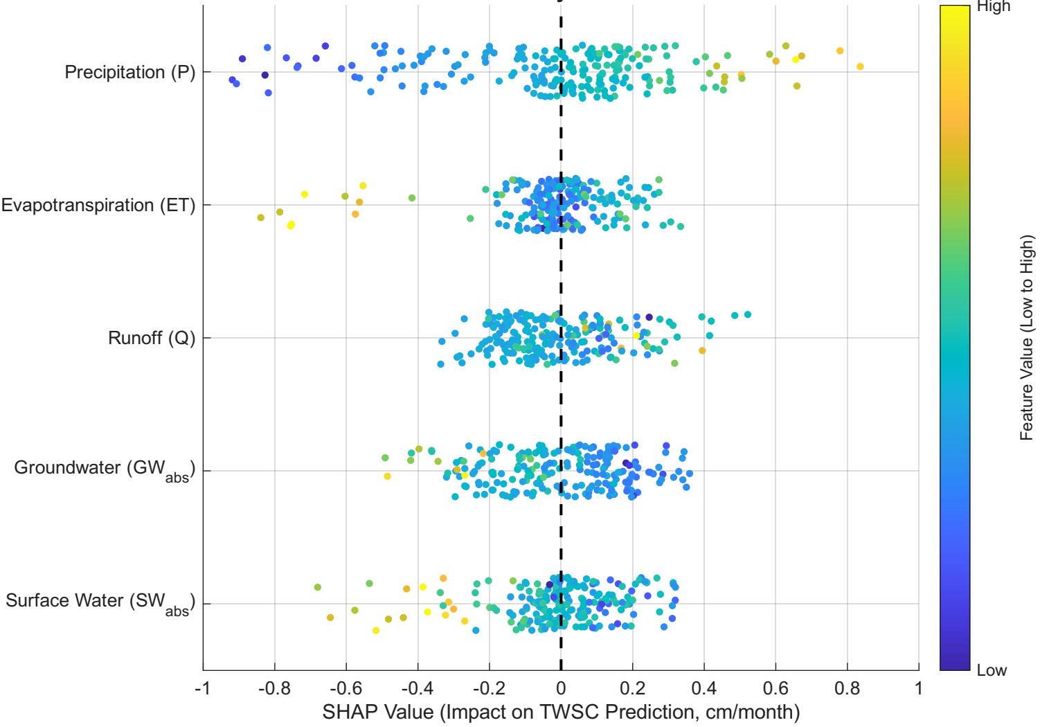
SHAP Summary Plot - Basin 39
