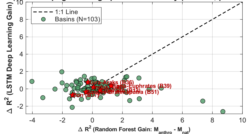
(b) Anthropogenic Fingerprint Consistency ( r = -0.26 , p < 0.001 )
