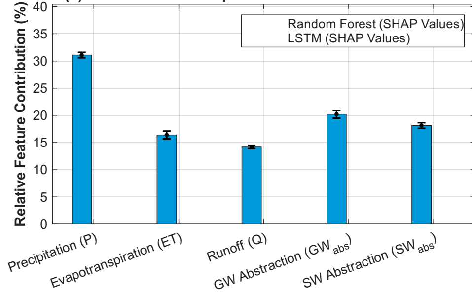
(c) Global Feature Importance Profiles across Drivers
