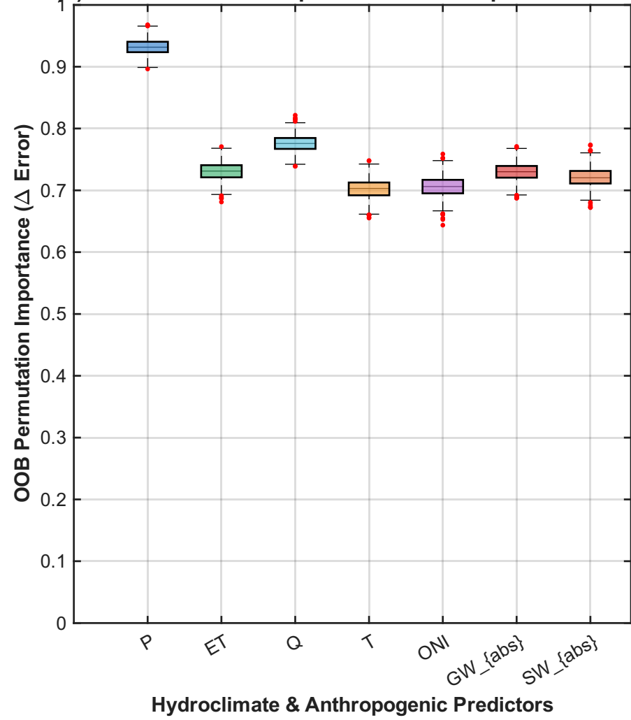
(b) Global Predictor Importance Bootstrap Distributions
