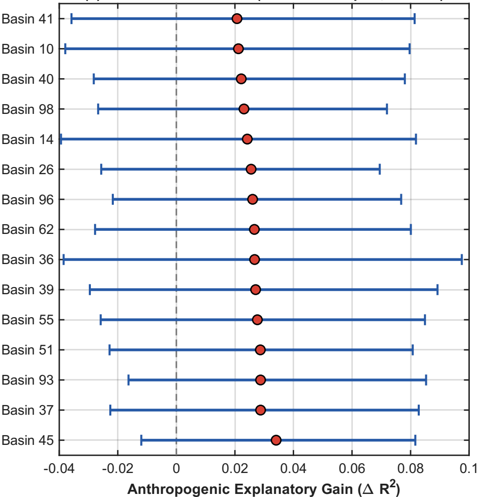
(a) \Delta R^2 Attribution Gain (95% Bootstrap CI, N=1000)
