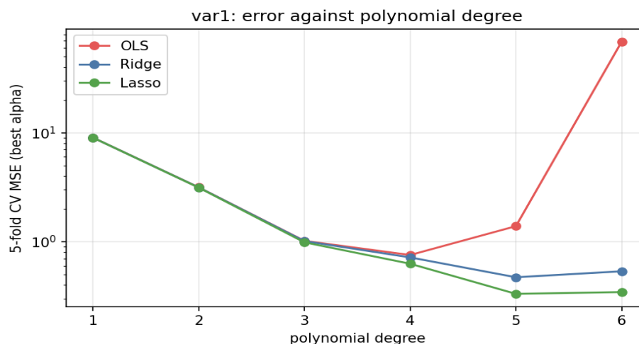
Figure 2. Var1 training-only cross-validated MSE against polynomial degree.
