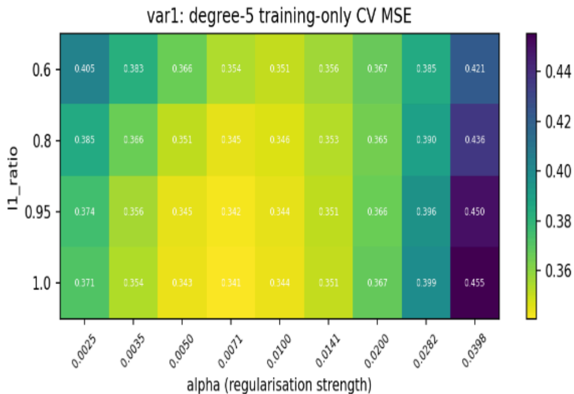
Figure 3. Var1 training-only CV MSE over alpha and l1_ratio at degree 5.
