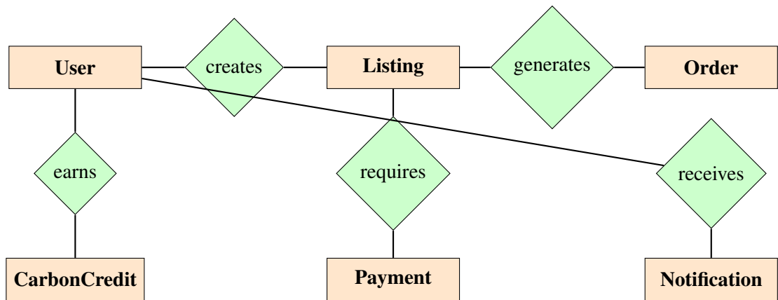
Figure 7.6: Entity-Relationship Diagram
