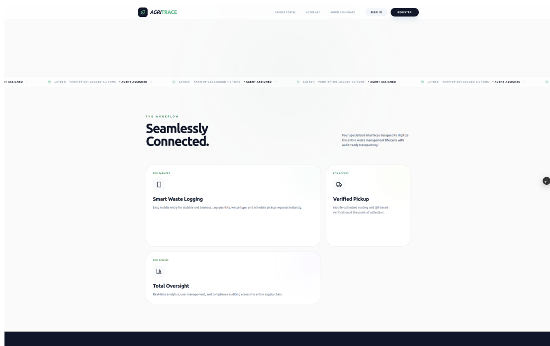
Figure 9.40: Features Page
