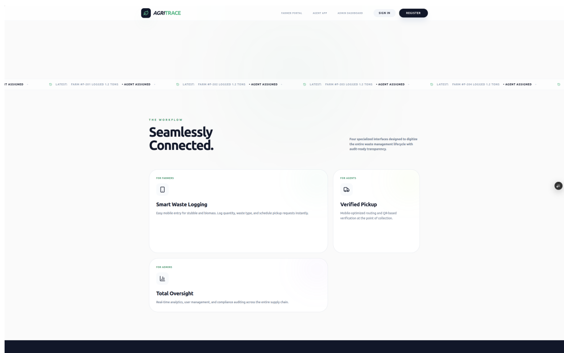
Figure 7.2: Features Section
