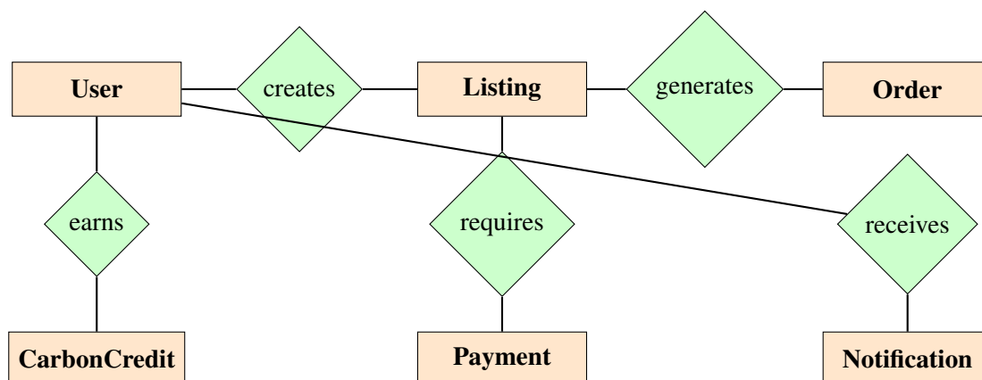
Figure 5.6: Entity-Relationship Diagram
