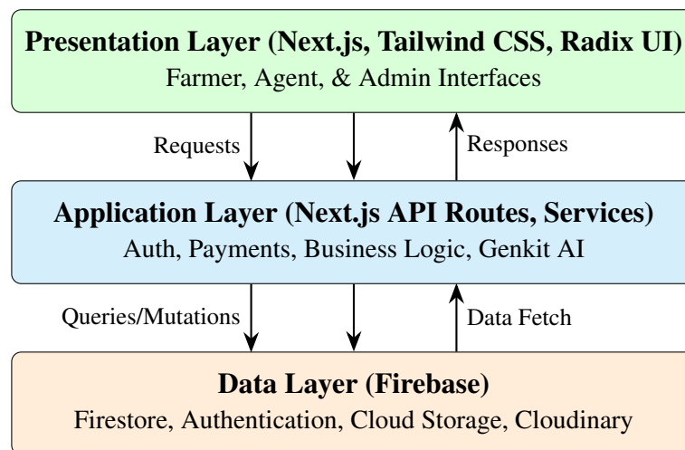
Figure 4.1: Three-Tier System Architecture
